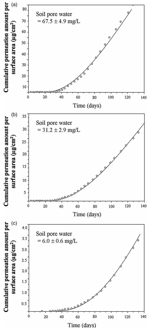
Figure 3 | Measured permeation data of benzene and curve fit data of permeation model: \circ , measured data; —, modeled curve.
