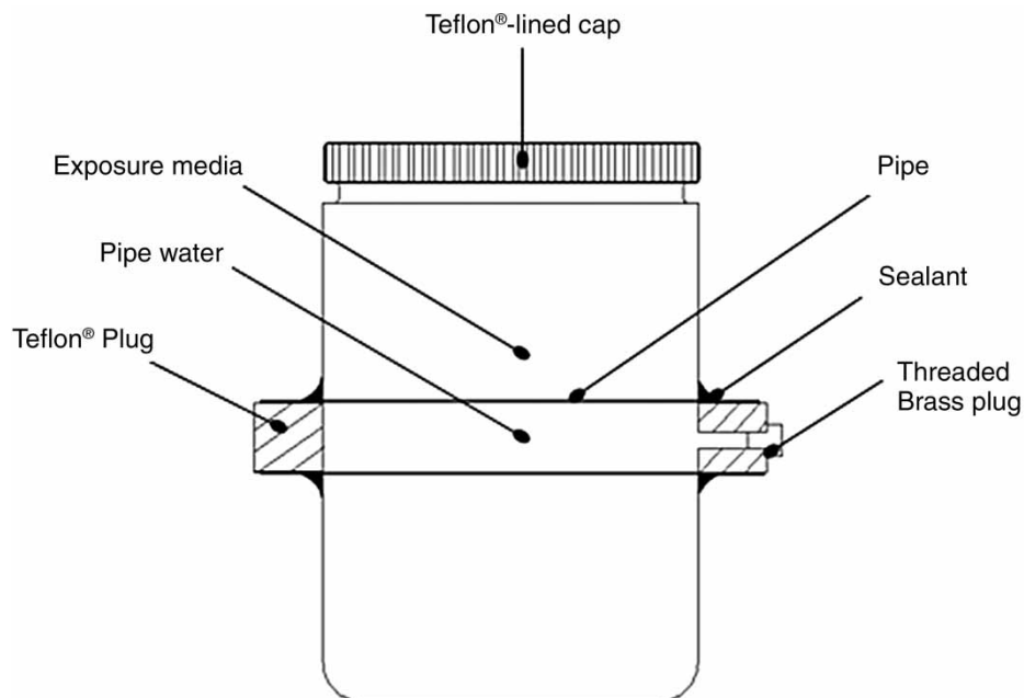
Figure 1 | Pipe-bottle apparatus.
