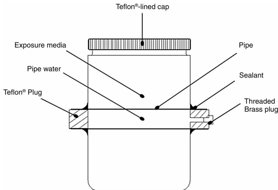
Figure 1 | Pipe-bottle apparatus.
