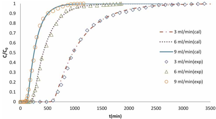
Figure 6 | Comparison of experimental breakthrough curves with different theoretical flow rates ( C_0 = 100 mg/L, L_0 = 10 cm).
