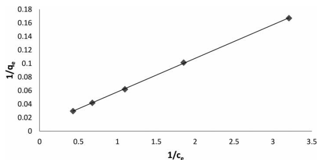
Figure 2 | Langmuir plot for adsorption of Pb(II) onto nanostructured \gamma -alumina. Conditions: adsorbent dose 5 g/L and pH 4.5.
