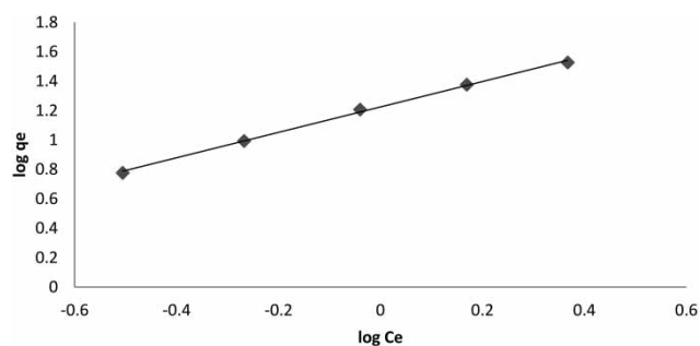
Figure 3 | Freundlich plot for adsorption of Pb(II) onto nanostructured \gamma -alumina. Conditions: adsorbent dose 5 g/L and pH 4.5.
