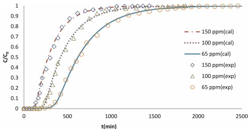
Figure 7 | Comparison of experimental breakthrough curves with different theoretical initial concentrations ( Q_0 = 6 mL/min, L_0 = 10 cm).
