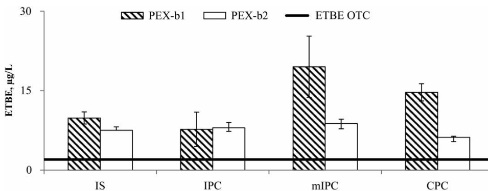
Figure 4 | ETBE results for two brands of PEX-b pipe were exposed to water for 3 days undergoing one of four cleaning methods. Shaded bar represents PEX-b1 pipe and white bar represents PEX-b2 pipe. Arithmetic mean and standard deviation values shown for ETBE concentration. The horizontal line for ETBE represents the concentration where people can detect an odor.
