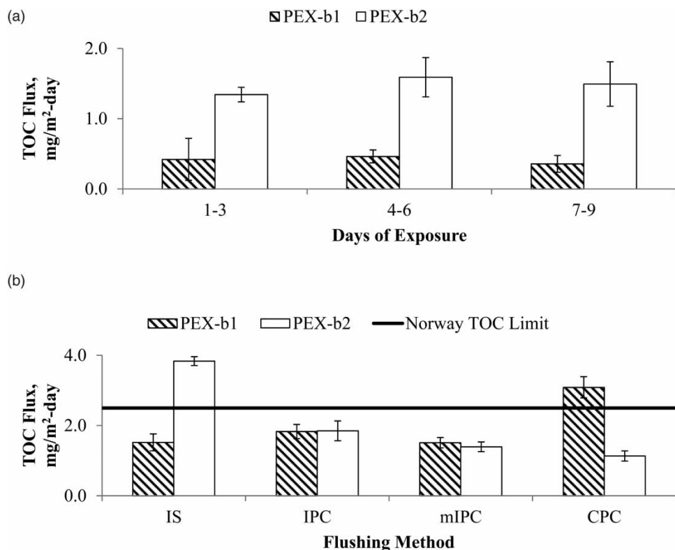
Figure 2 | Comparison of mean TOC flux from (a) two brands of PEX-b pipe exposed to water over 9 days with water changes every 3 days and (b) two brands of PEX-b pipe exposed to water for 3 days undergoing one of four cleaning methods. The shaded bar represents PEX-b1 pipe and the white bar represents PEX-b2 pipe. Arithmetic mean and standard deviation values are shown for TOC. The horizontal line for the TOC graph represents the Norwegian limit for TOC flux. There are no guidelines for TOC flux in the USA.
