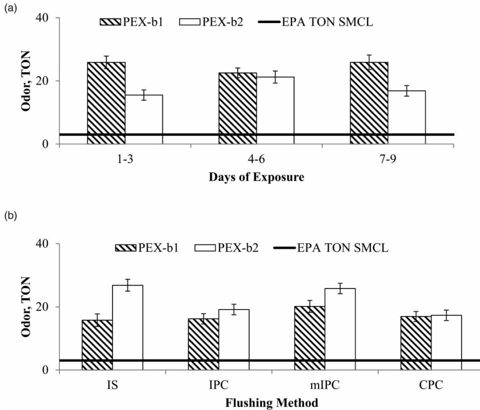
Figure 3 | Comparison of mean TON from (a) two PEX-b pipe brands exposed to water over 9 days with water changes every 3 days and (b) two PEX-b pipe brands exposed to water for 3 days after undergoing one of four cleaning methods. PEX-b1 pipe (shaded bar), PEX-b2 pipe (white bar); geometric mean and standard deviation values are shown. The horizontal line represents the USEPA SMCL = 3 TON.
