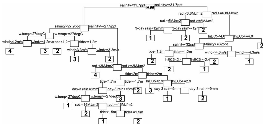
Figure 7 | Structure of the four-category CT for Big Wave Bay in the post-HATS period. Note: in the end-leaves, ‘1’ to ‘4’ correspond to BWQI-1 to 4, respectively.
