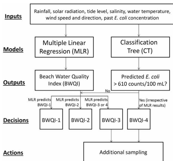
Figure 8 | Flow diagram of the proposed operation rules for beach management using a combined MLR and CT modelling approach.
