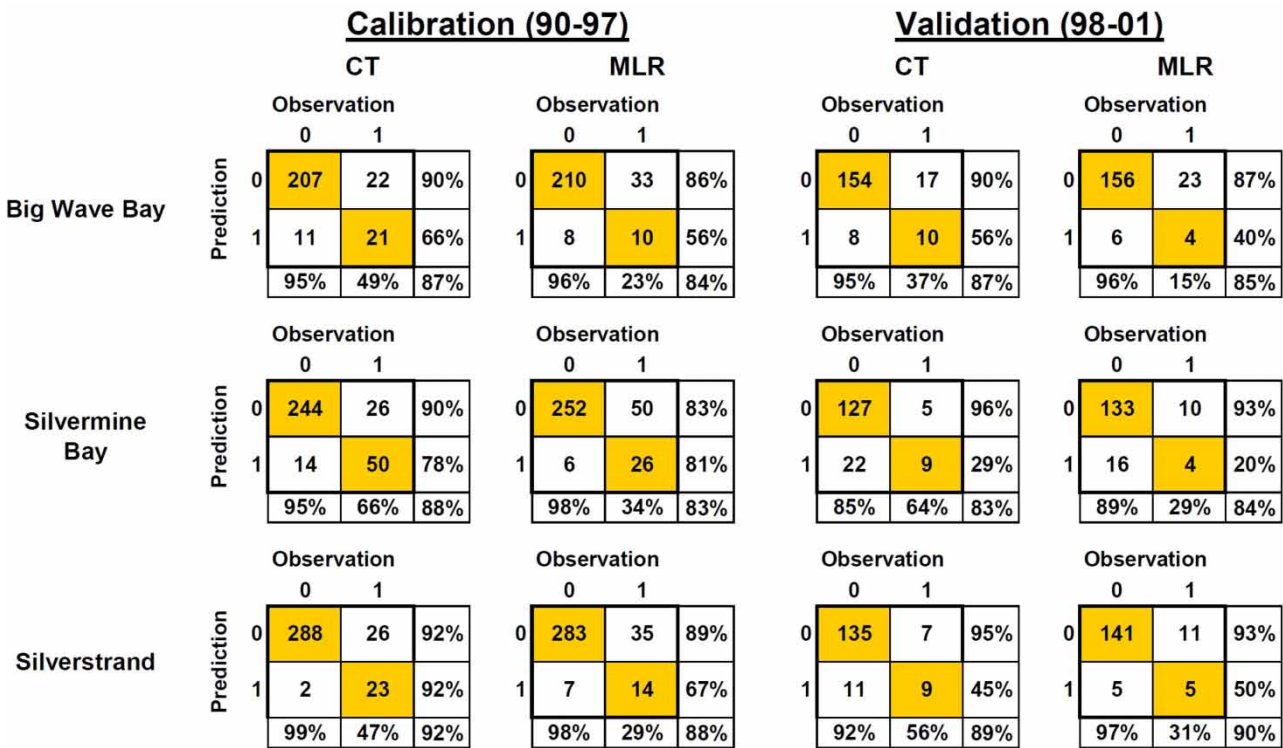
Figure 2 | CT and MLR model performances in the pre-HATS period: calibration period (1990–1997) and validation period (1998–2001). Note: in the table, ‘1’ = 610 threshold exceedance; ‘0’ = 610 threshold non-exceedance.
