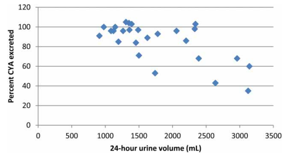
Figure 3 | Plot of percent CYA excreted versus 24 hour urine volume.
