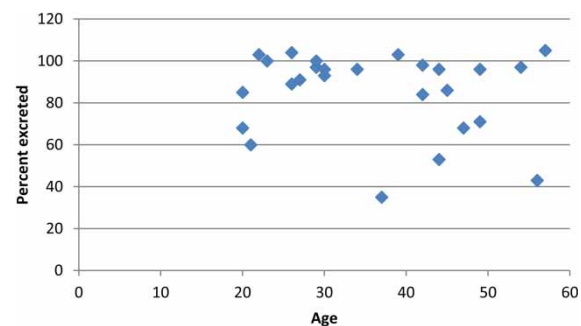
Figure 4 | Plot of percent CYA excreted versus participant age in years.
