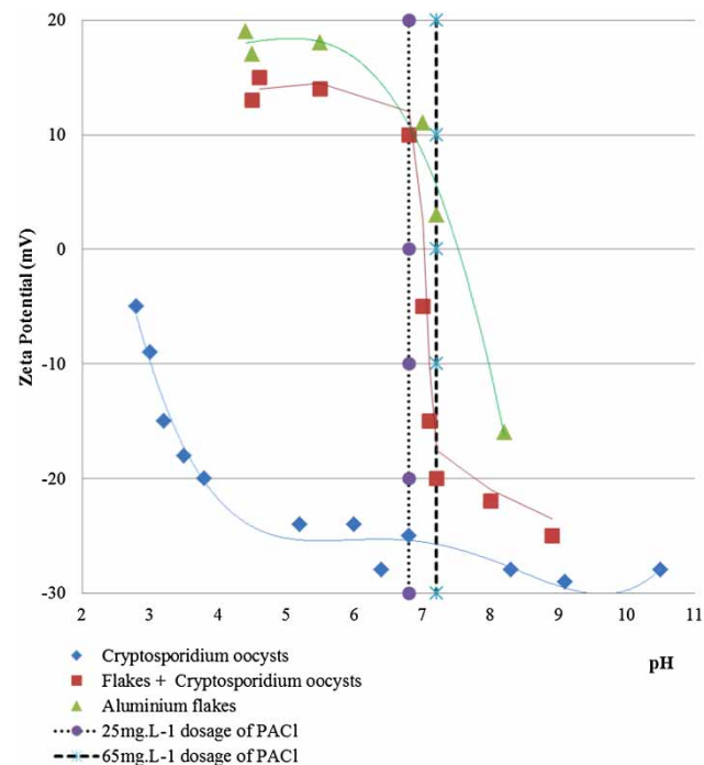
Figure 1 | Effect of pH on the zeta potential of the flakes, oocysts, and oocysts/flakes conjugate (Bustamante et al. 2001). The vertical lines represent the pH coagulation for the 25 mg L -1 and 65 mg L -1 dosages analyzed in this study.
