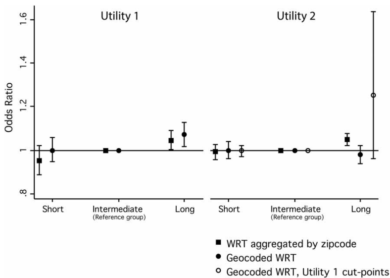
Figure 2 | Comparison of results of logistic regression models using different approaches to exposure assessment. Odds ratio (OR) estimates and 95% confidence intervals are shown for Utility 1 and Utility 2 for the association between water residence time (WRT) and visits to the ED for GI illness. WRT was classified as 'Short' ( \leq 10 th percentile), 'Intermediate' (11th–89th percentile), or 'Long' ( \geq 90 th percentile). Squares indicate OR using WRT aggregated by ZIP code, as reported by Tinker et al. (2009). Circles indicate OR using geocoded WRT, with address of patient matched to WRT of nearest node. Closed circles represent OR using the intermediate WRT category of each utility as its own reference. Open circles represent OR for Utility 2 relative to the WRT category percentile cut-off values of Utility 1. Models controlled for Medicaid status, median household income at the census block level, percentage minority at the census block level, patient age, Euclidean distance between the hospital where the ED visit occurred and the geocoded patient residence, indicator variables for hospital, year, day-of-week, season, and product terms for age*hospital, age*distance to hospital, age*Medicaid status.
