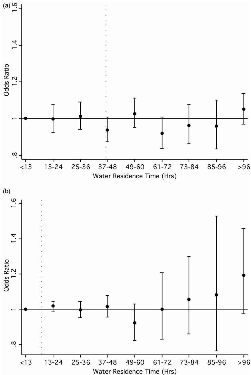
Figure 3 | Results of logistic regression models examining the relationship between WRT (12-h increments) vs. ED visits for GI illness. Odds ratio (OR) estimates and 95% confidence intervals are shown for (a) Utility 1 and (b) Utility 2, using geocoded WRT estimates, with address of patient matched to WRT of nearest node. Reference condition for each estimate is <12 h. Mean WRT for each utility is shown with a dotted line. Models controlled for Medicaid status, median household income at the census block level, percentage minority at the census block level, patient age, Euclidean distance between the hospital where the ED visit occurred and the geocoded patient residence, indicator variables for hospital, year, day-of-week, and product terms for age*hospital, age*distance to hospital, age*Medicaid status.
