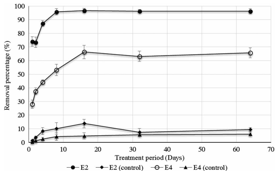
Figure 9 | Removal of Ni 2+ ions in E2 and E4 by Bacillus subtilis 2012WTNC during the bioaugmentation process of four types of secondary effluents conducted at 45 °C for 64 days: E2, secondary effluent containing 10 mg Ni 2+ L -1 ; E4, secondary effluent containing 10 mg Ni 2+ L -1 and 1 g cephalaxin L -1 . Error bars represent the standard deviation from the mean.
