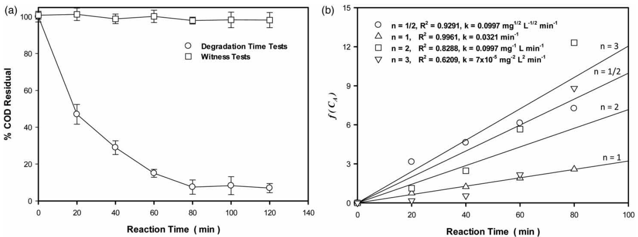
Figure 3 | (a) Profile of COD removal under the conditions of treatment 6. (b) Apparent kinetic coefficient: for n = 1/2 and n = 1 , f(C_{t_1}) = corresponding; for n = 2 , the k value is divided by 100 and for n = 3 , it is divided by 1,000.
