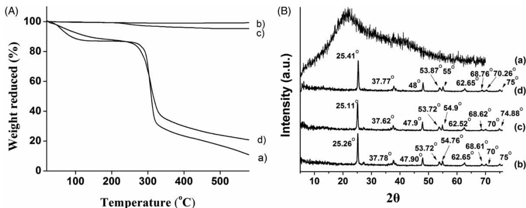
Figure 4 | (A) TGA curves. (a) starch, (b) UTi, (c) CMT, (d) SPC. (B) XRD spectra. (a) starch, (b) UTi, (c) CMT, (d) SPC.
