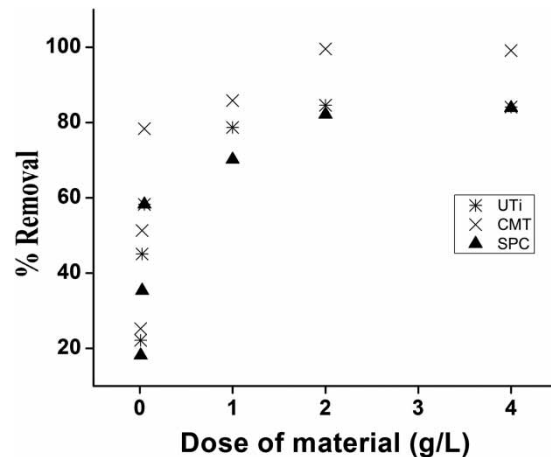
Figure 5 | Efficacy of UTi, CMT and SPC for As(V) removal.
