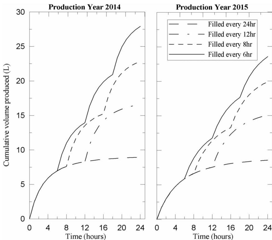
Figure 5 | Model prediction of cumulative volume of water produced, V(t) , if filters are refilled once per day (every 24 h), twice per day (every 12 h), three times per day (every 8 h) and four times per day (every 6 h). After Schweitzer et al. (2013).
