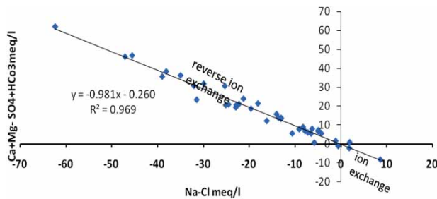
Figure 8 | Relationship between Ca + Mg-HCO 3 -SO 4 versus Na-Cl for the Quaternary aquifer samples.
