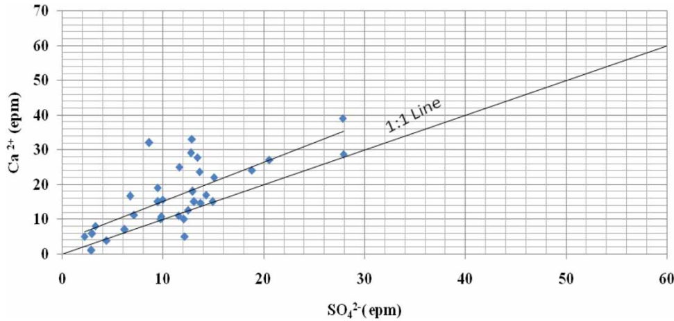
Figure 7 | Ca 2+ vs SO 4 2- relationship.
