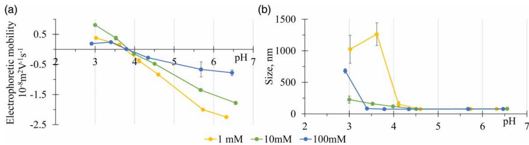
Figure 3 | Measurement of electrophoretic mobility (a) and size distribution (b) of 28B phage under varying ionic strengths ( \text{NaNO}_3 ) and pH conditions; measurements are expressed as mean values ( n = 3 ) and SEM (standard error of the mean).
