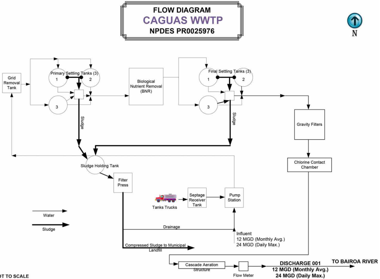
Figure 2 | Flow chart of the Caguas WWTP ( www.epa.gov/region02/water/permits.html ).
