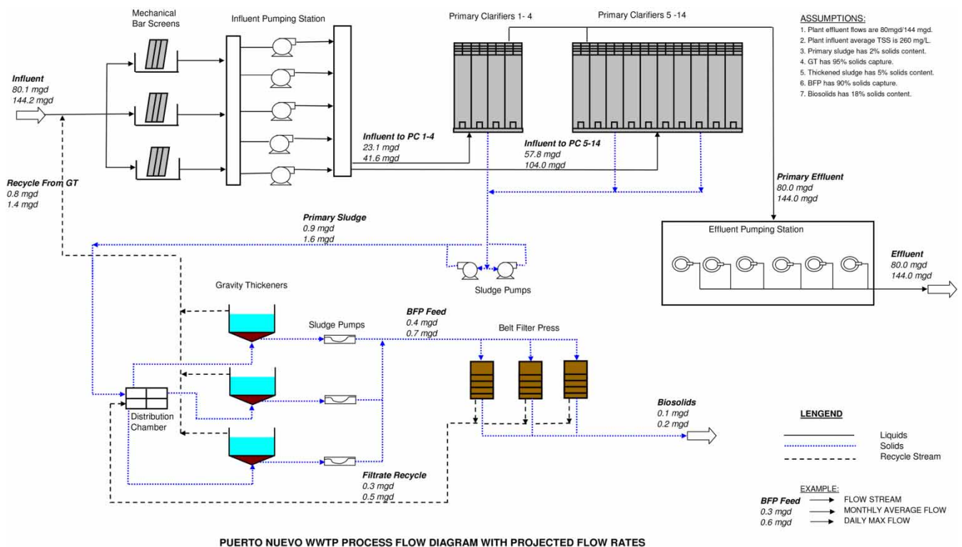
Figure 1 | Flow chart of the Puerto Nuevo WWTP ( www.epa.gov/region02/water/permits.html ).
