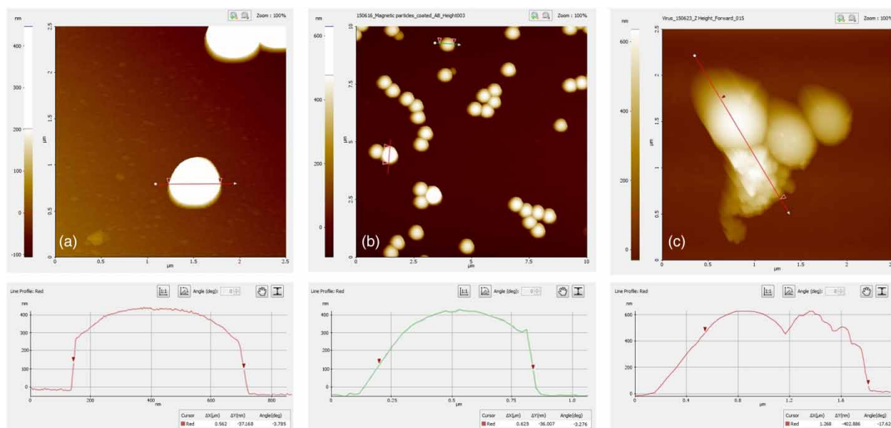
Figure 3 | AFM images: (a) fluoromagnetic particles; (b) functionalized particles; (c) biofunctionalized magnetic particles after exposure to 10^6 VP/L of rotavirus.
