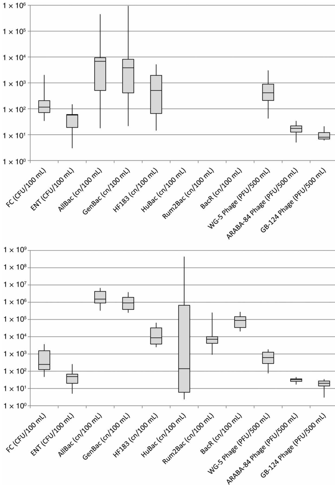
Figure 2 | MST and water quality indicator concentrations at Sonceboz (above) and Tavannes (below) sampling sites. Within-box solid lines represent the median, upper and lower edges of the box represent third and first quartiles, and upper and lower whiskers represent maximum and minimum values, respectively.
