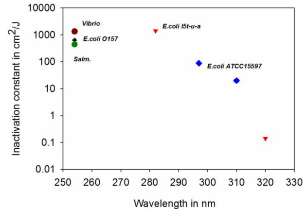
Figure 7 | Bacterial action spectra: ◆ E. coli ATCC15597, ● Vibrio , ■ Salmonella , ◆ E. coli O157 from Hijnen & Medema (2005); ▼ E. coli I5t-u-a Boyce & Setlow (1963).
