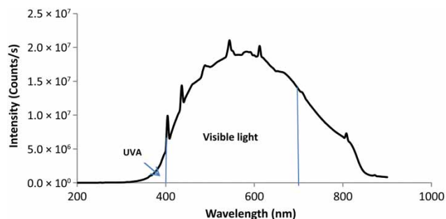
Figure 2 | Incandescent lamp output spectrum measured using a spectrofluorometer (Horiba, FluoroLog-3). Note: Intensity units from the instrument are interpreted as arbitrary units or counts per second.
