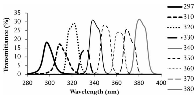
Figure 1 | Transmittance spectra of narrow bandpass optical filters used in this research.
