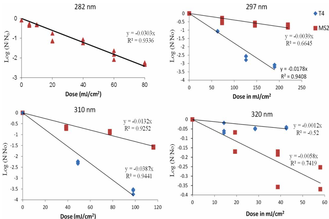
Figure 4 | Dose-response curve for MS2 at 282 nm and MS2 and T4 at 297 nm, 310 nm, and 320 nm.
