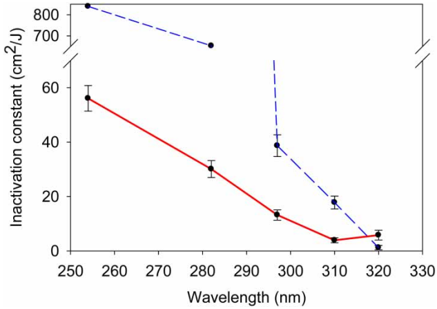
Figure 5 | Action spectra for MS2 (continuous line), T4 (dashed line). T4 inactivation constants at 254 nm and 282 nm were deduced from Fallon et al. (2007) and Winkler et al. (1962), respectively.
