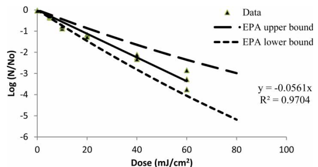
Figure 3 | Dose-response behavior for coliphage MS2 at 254 nm. Upper and lower bounds for UV 254 dose-response behavior of MS2, as defined by USEPA (2006) are included for reference.
