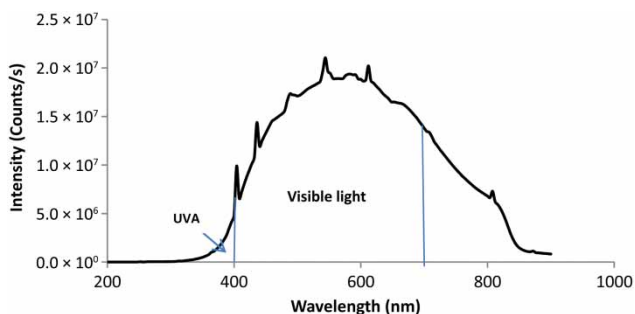
Figure 2 | Incandescent lamp output spectrum measured using a spectrophotometer (Horiba, FluoroLog-3). Note: Intensity units from the instrument are interpreted as arbitrary units or counts per second.
