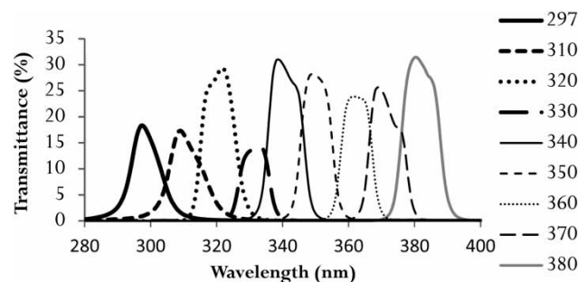
Figure 1 | Transmittance spectra of narrow bandpass optical filters used in this research.
