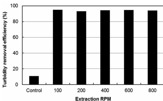
Figure 1 | Turbidity removal efficiency by rotation speed of MO seed extraction (Extraction condition: 5 g MO/100 mL, 100–800 rpm, 30 min, Dose of MO seed extract: 10 mL/L).
