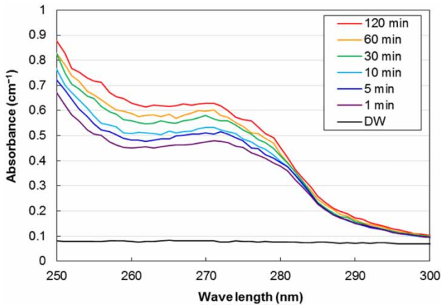
Figure 6 | Absorbance of MO seed extract by extraction time (Extraction condition: 5 g MO/100 mg, 100 rpm, 1–120 min time).
