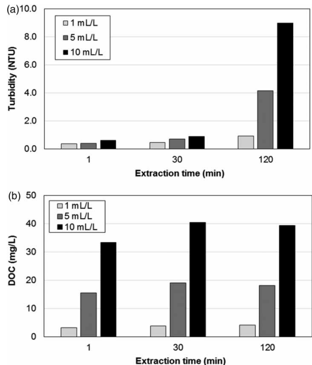
Figure 8 | Turbidity (a) and DOC (b) with adding the MO seed extract by extraction time to distilled water (Extraction condition: 5 g MO/100 mL, Extract dose: 1, 5, and 10 mL/L, Extraction time: 1, 30, and 120 min).
