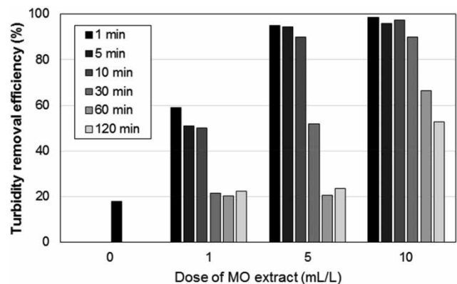
Figure 2 | Turbidity removal efficiency in coagulation test using MO seed extract made by various extraction time (Extraction condition: 5 g MO/100 mL, 100 rpm, 1–120 min, Dose of MO extract: 1–10 mL/L).
