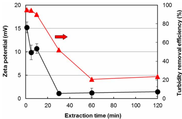
Figure 4 | Zeta potential of MO seed extract made by various extraction time (Extraction condition: 5 g MO/100 mL, 100 rpm, 1–120 min, Dose of MO extract: 5 mL/L).
