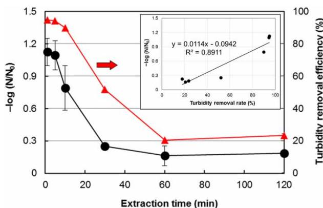
Figure 3 | Removal of E. coli in coagulation test using MO seed extract (Extraction condition: 5 g MO/100 mL, 100 rpm, 1–120 min, Dose of MO extract: 5 mL/L).
