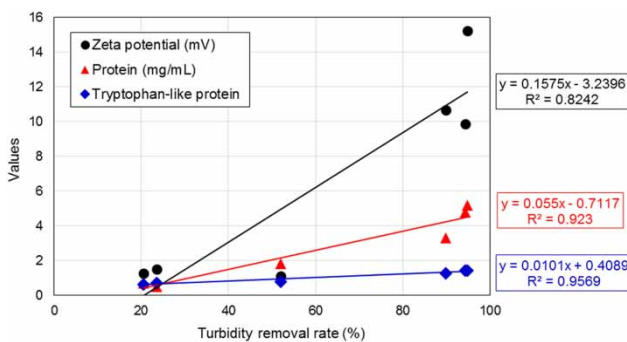
Figure 7 | Correlation of turbidity removal rate with zeta potential, protein, and tryptophan.
