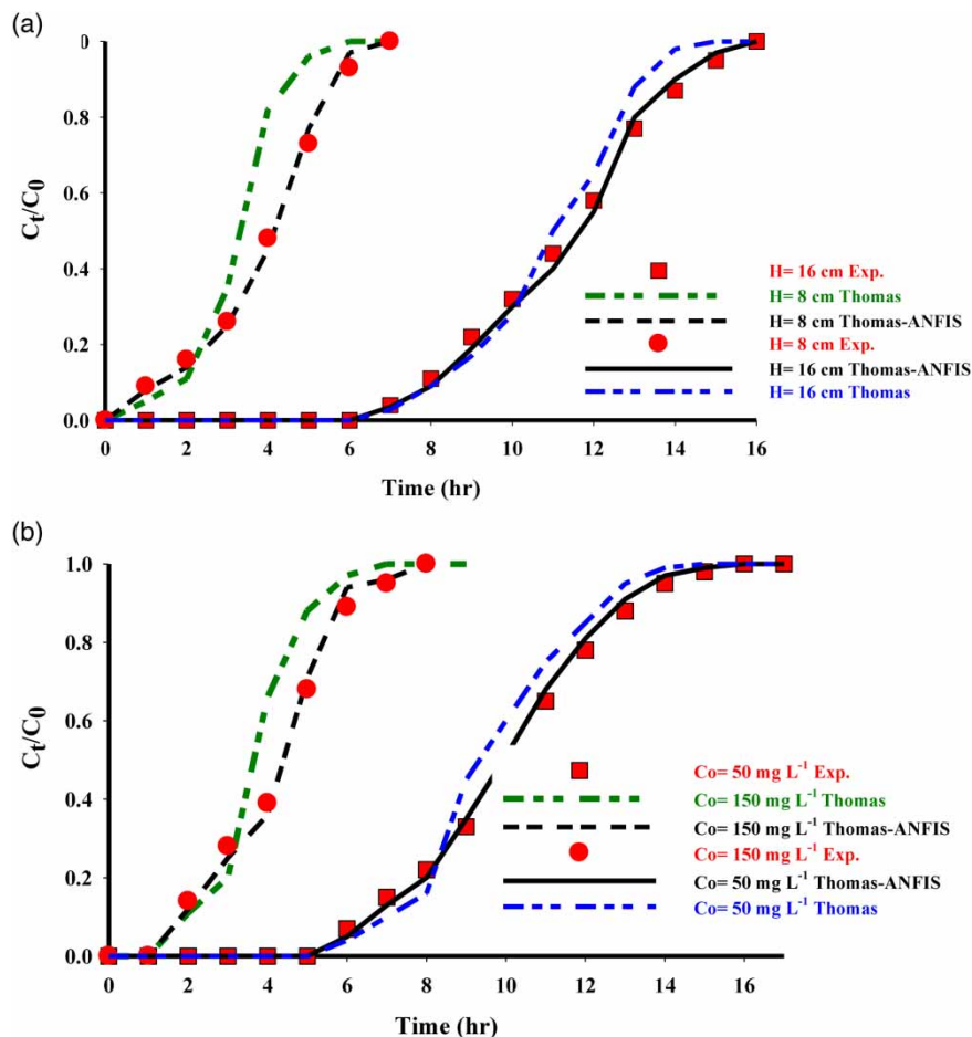
Figure 4 | Measured and predicted BTC of Cd(II) ions acquired by Thomas and hybrid models: (a) temperature, 25 \pm 1 °C; influent concentration, 100 \text{ mg L}^{-1} ; influent flow rate, 1.5 \text{ mL min}^{-1} ; pH, 7; (b) temperature, 25 \pm 1 °C; bed height, 12 cm; influent flow rate, 1.5 \text{ mL min}^{-1} ; pH, 7.
