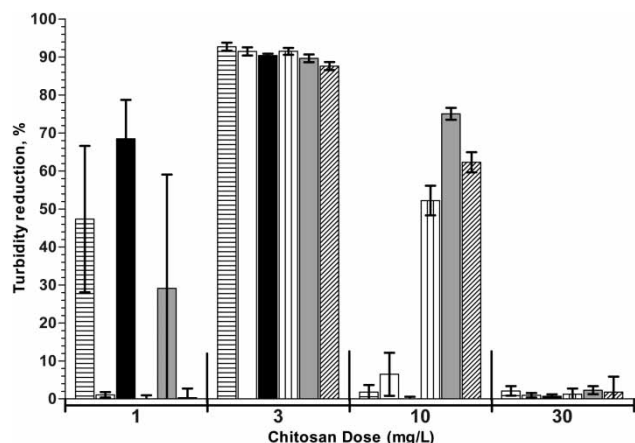
Figure 4 | Effects of polymer degree of deacetylation (5 mPa·s viscosity) on kaolinite turbidity reduction (horizontal stripes = 70% DD; white = 75%; black = 80%; vertical stripes = 85%; gray = 90%; diagonal stripes = 95%; bars = 95% CI).
