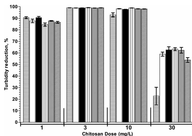
Figure 3 | Effects of polymer degree of deacetylation (5 mPa·s viscosity) on bentonite turbidity reduction (horizontal stripes = 70% DD; white = 75%; black = 80%; vertical stripes = 85%; gray = 90%; diagonal stripes = 95%; bars = 95% CI).
