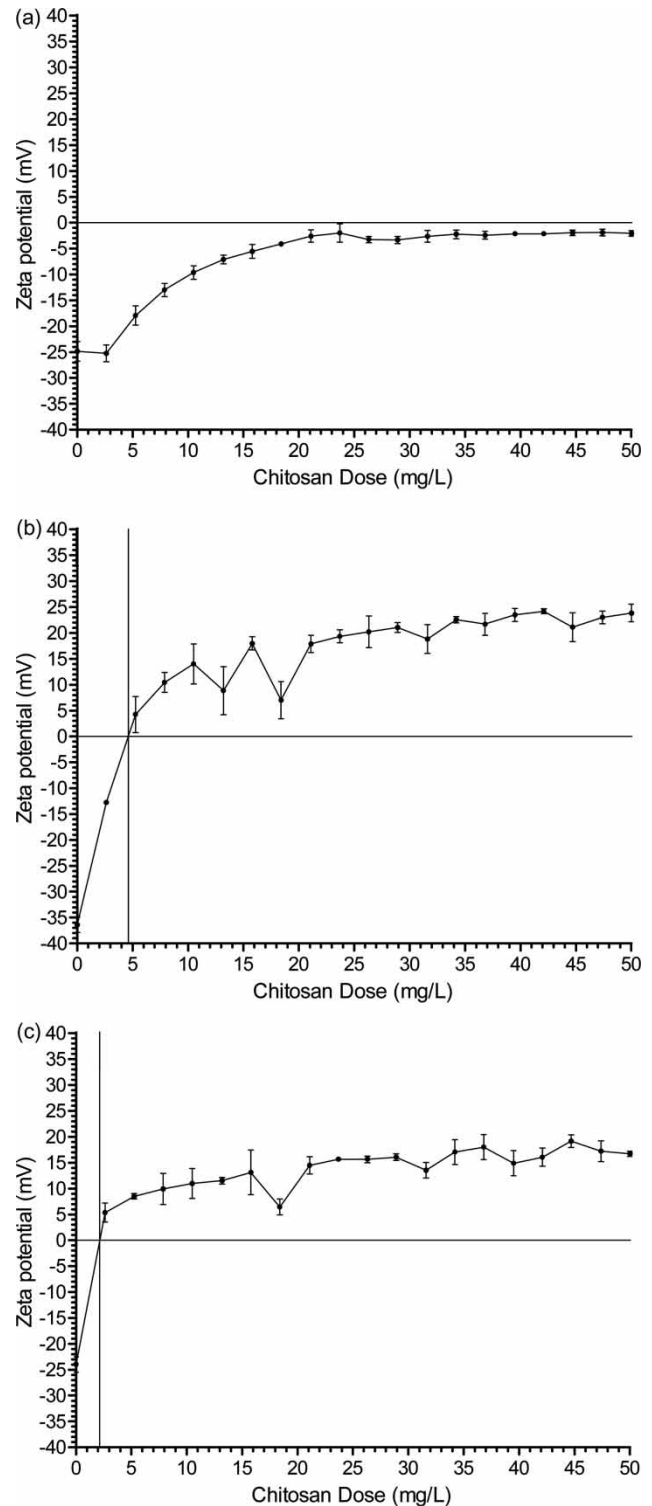
Figure 7 | Zeta potentials and points of zero charge (PZCs) of kaolinite turbidity coagulation by (a) chitosan MW 5,000 Da, (b) MW 100,000 Da, and (c) 70% DD (black circles mean zeta potential; connecting line = weighted mean zeta potential; vertical line = PZC; bars = 95% CI).
