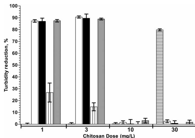
Figure 2 | Effect of chitosan MW (chitosans of 90% DD) and dose on reduction of kaolinite turbidity (horizontal stripes = 5,000 Da; white = 50,000 Da; black = 100,000 Da; vertical stripes = 600,000 Da; gray = 1,000,000 Da; bars = 95% CI).
