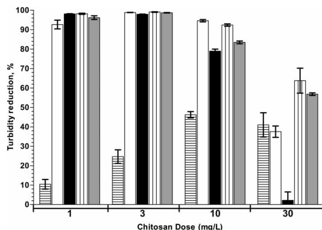
Figure 1 | Effects of chitosan MW (chitosans of 90% DD) and dose on bentonite turbidity reduction (horizontal stripes = 5,000 Da; white = 50,000 Da; black = 100,000 Da; vertical stripes = 600,000 Da; gray = 1,000,000 Da; bars = 95% CI).
