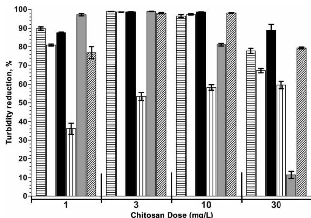
Figure 5 | Effects of polymer modification by functional groups (DD 80–95%, viscosity 2–300 mPa·s) on bentonite turbidity reduction (horizontal stripes = acetate; white = lactate; black = HCl; vertical stripes = carboxymethyl; gray = acetate-SK; diagonal stripes = lactate-SK; bars = 95% CI).
