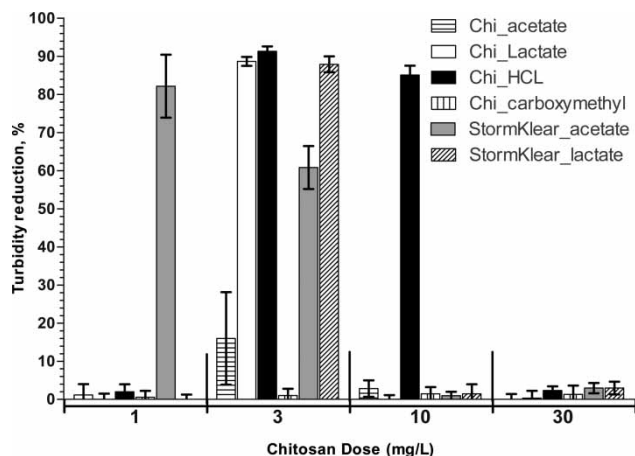
Figure 6 | Effects of polymer modification by functional groups (DD 80–95%, viscosity 2–300 mPa·S) on kaolinite turbidity reduction (horizontal stripes = acetate; white = lactate; black = HCl; vertical stripes = carboxymethyl; gray = acetate-SK; diagonal stripes = lactate-SK; bars = 95% CI).
