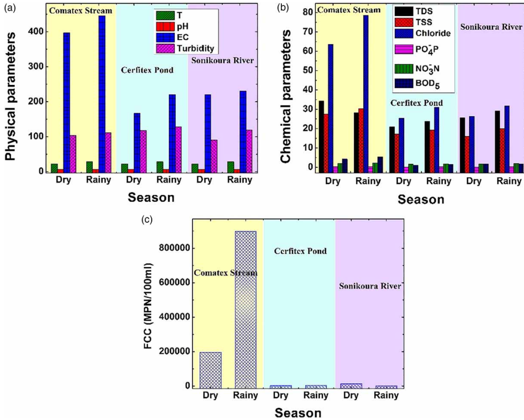
Figure 3 | Seasonal variations in some physical, chemical and bacteriological parameters in the water sample from the three water bodies.
