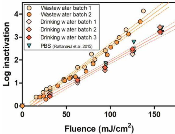
Figure 3 | Human adenovirus genotype five (HAdV-5) inactivation profiles of different water samples. Dashed lines show 95% confidence intervals.
