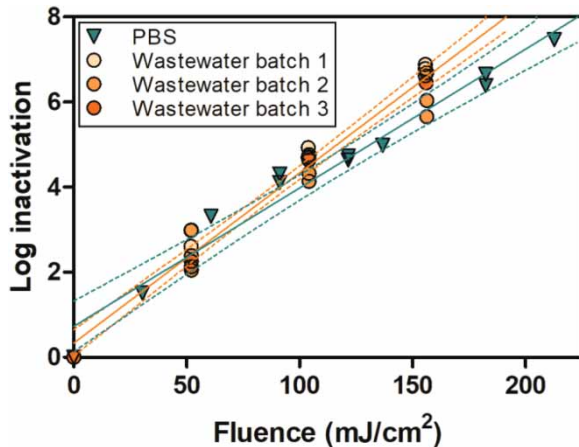
Figure 4 | Bacteriophage MS-2 inactivation profiles of PBS and wastewater samples. Dashed lines show 95% confidence intervals.
