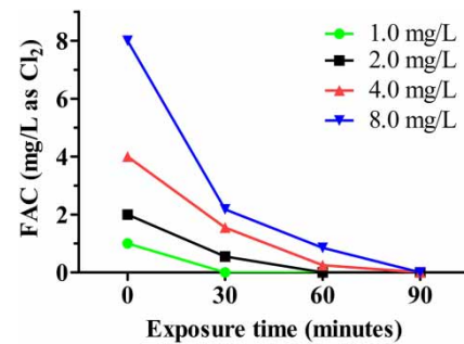
Figure 1 | Concentration of FAC in water during NaOCl photolysis by UV-C ( 243 \mu\text{W}\cdot\text{cm}^2/\lambda = 254 \text{ nm} ).
