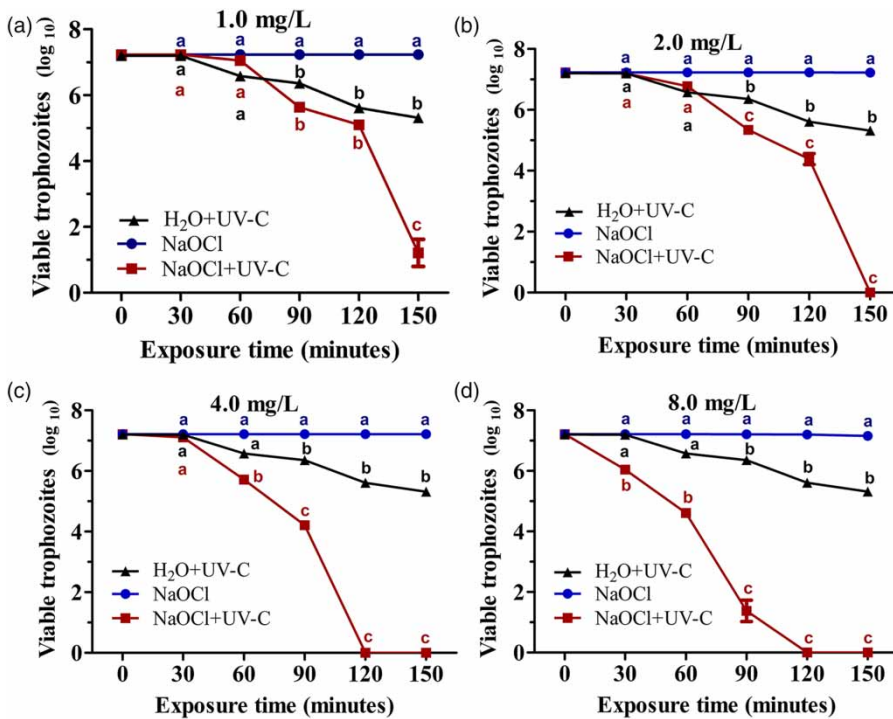
Figure 3 | Effect of photolysis of different doses of NaOCl by UV-C radiation ( 243 \mu\text{W}\cdot\text{cm}^2/\lambda = 254 \text{ nm} ) on the viability of A. castellanii trophozoites. The results are expressed as the average number of trophozoites per mL. Points with different letters indicate significant differences ( p < 0.05 ).
