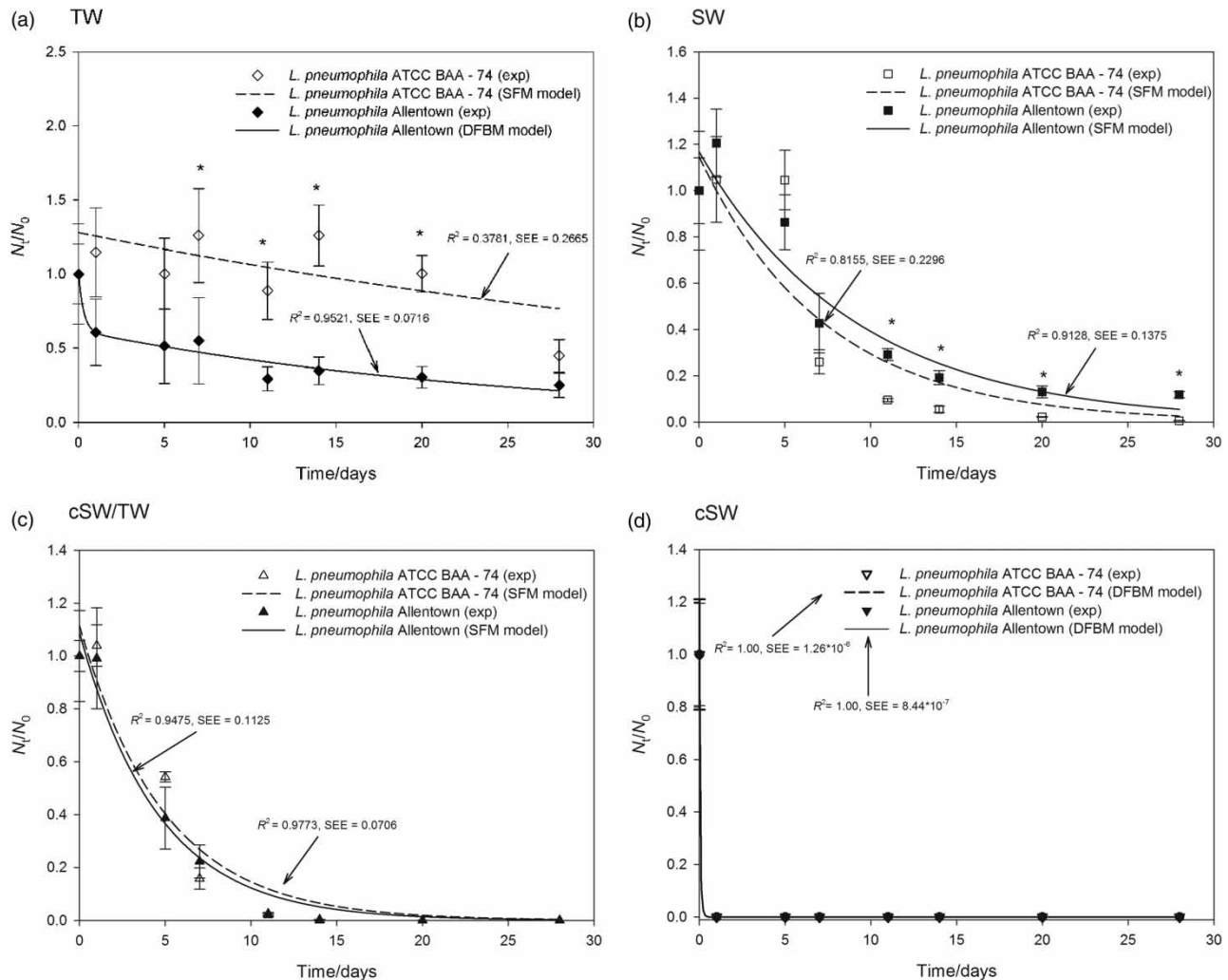
Figure 2 | Reduction of L. pneumophila ATCC BAA-74 and Allentown strains in (a) tap water (TW), (b) sea water (SW), (c) chlorinated sea water/tap water (cSW/TW, 50:50 ratio) and (d) chlorinated sea water (cSW). Symbols represent the experimental data, while lines represent the theoretical curves described by the Single First-Order (SFM) and Double First-Order Exponential Biphasic (DFBM) kinetics mathematical models. Data are expressed as mean \pm standard deviation (at least five replicates).
