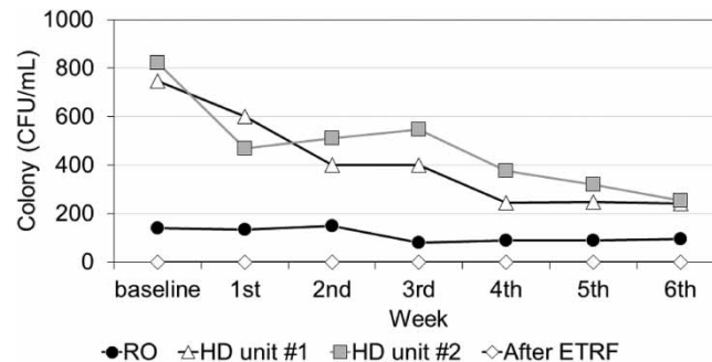
Figure 5 | Changes in microbial colony counts. The baseline of microbial colony counts of HD units #1 and #2 were 747 and 823 CFU/mL, respectively. After 6 weeks, the microbial colony counts of both #1 and #2 HD units decreased to 67.6 and 69.1%, respectively.
