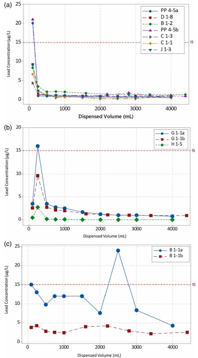
Figures 4 | (a–c) Variability in lead concentrations with dispensed volume.
