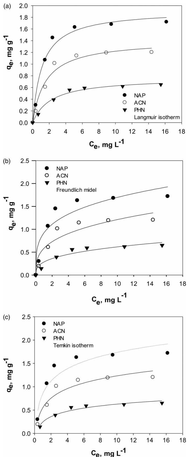
Figure 6 | Langmuir, Freundlich, and Temkin isotherms for NAP, ACN, and PHN adsorption onto NH 2 -SBA-15 (conditions: pH 5, dosage 3 \text{g L}^{-1} , temperature 25 °C).
