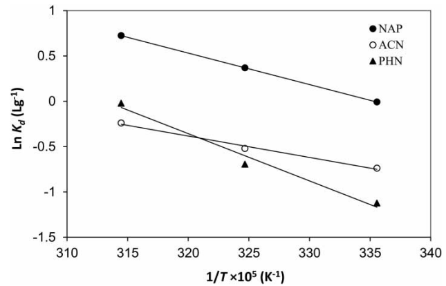
Figure 9 | Plots of \ln K_d versus 1/T for NAP, ACN, and PHN adsorption onto NH 2 -SBA-15 (conditions: adsorbent dose 3 g L -1 , pH 5, initial concentration of NAP, ACN, and PHN of 6, 6, and 4 mg L -1 , respectively).
