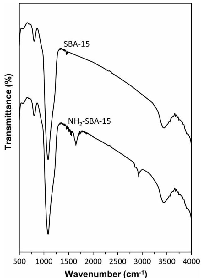
Figure 3 | FTIR spectra of SBA-15 and NH 2 -SBA-15.
