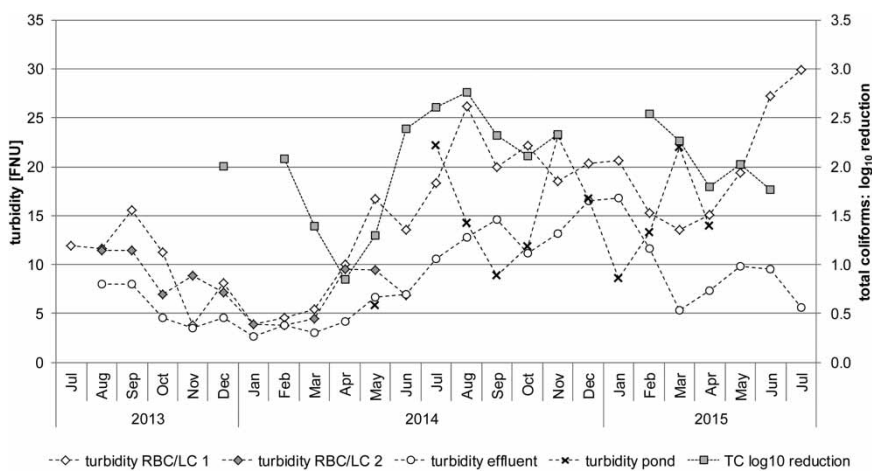
Figure 2 | Turbidity in the effluent of the rotating biological contactors and lamella clarifiers (RBC/LC 1 and 2), after passing the microscreen (effluent) and in the storage pond and log 10 reduction of TC.
