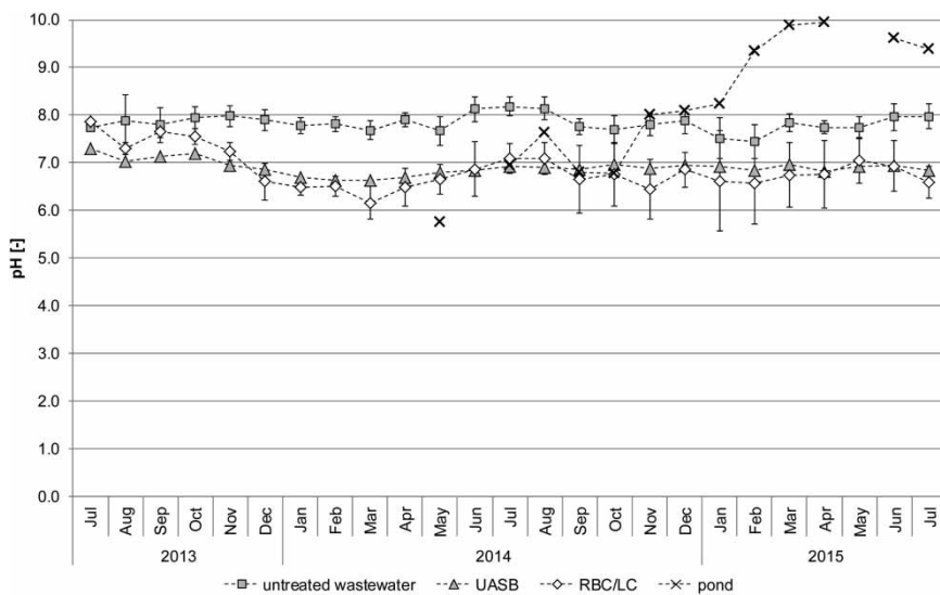
Figure 3 | pH in the untreated wastewater, after sedimentation and anaerobic pretreatment (UASB), after aerobic treatment and separation of solids via lamella clarifiers (RBC/LC) and in the storage pond (bars represent standard deviation of the mean).
