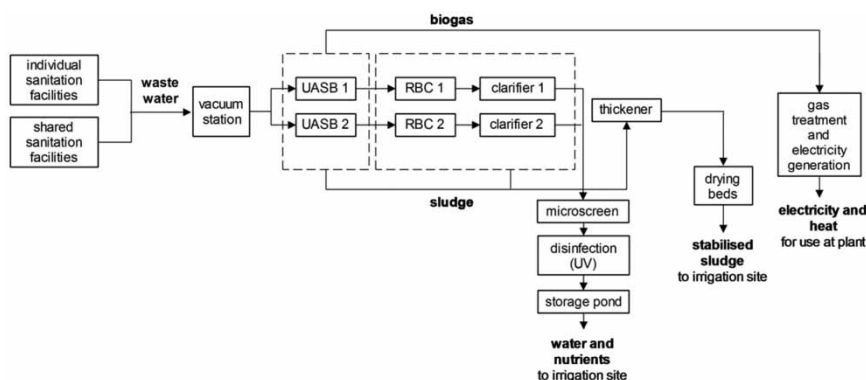
Figure 1 | Schematic drawing of the sanitation and water reuse project.
