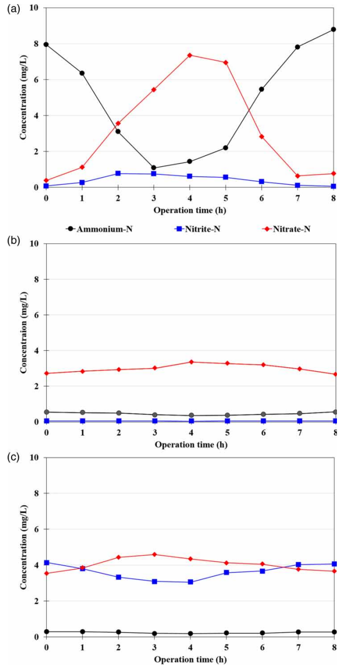
Figure 6 | Change of \text{NH}_4\text{-N} , \text{NO}_2\text{-N} and \text{NO}_3\text{-N} in (a) concrete reactor, (b) sponge reactor, (c) commercial carrier reactor.
