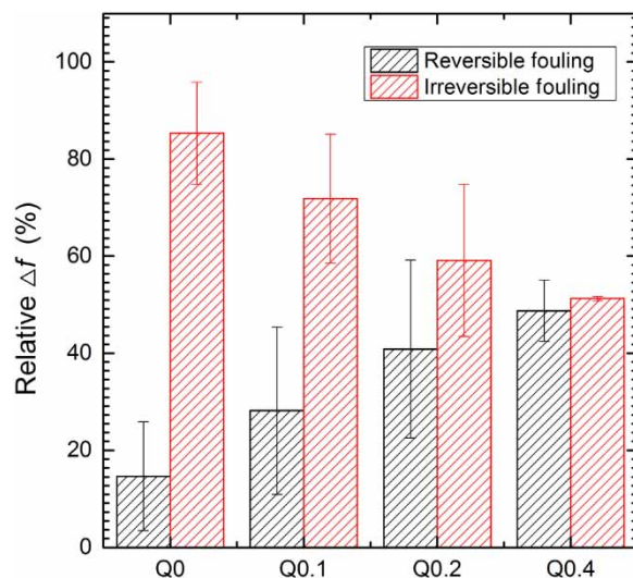
Figure 6 | Relative \Delta f of adsorbed bacteria on Q0, Q0.1, Q0.2, and Q0.4 sensors after introducing DI water (i.e., reversible fouling and irreversible fouling), respectively. Error bars represent standard deviations of at least three runs.
