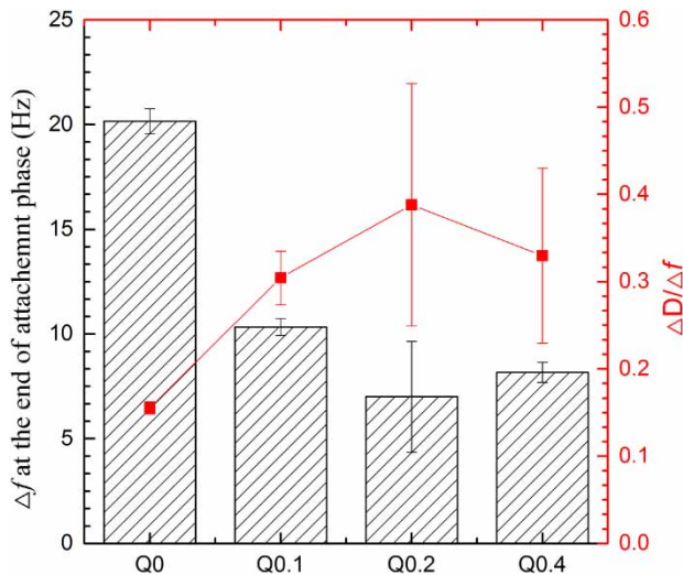
Figure 1 | Change of frequency ( \Delta f ) and |\Delta D/\Delta f| values at the end of bacterial attachment phase and for Q0, Q0.1, Q0.2, and Q0.4 coated quartz crystals sensors. Error bars represent standard deviations of at least three runs.
