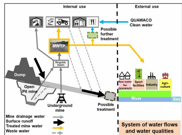
Figure 2 | Generalized mine water system.
