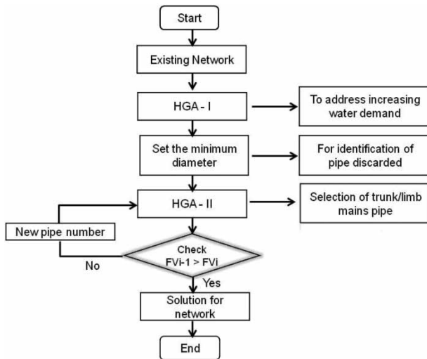
Figure 4 | Methodology of HGA I and II.
