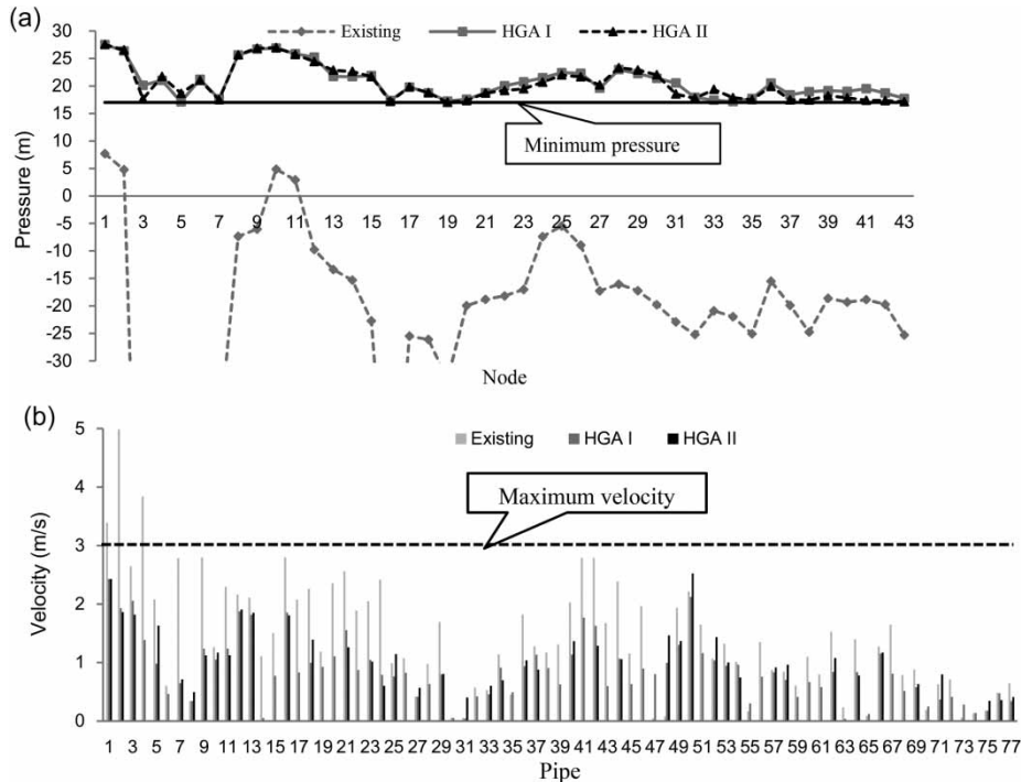
Figure 6 | Hydraulic analysis: (a) pressure at node; (b) velocity at pipe.
