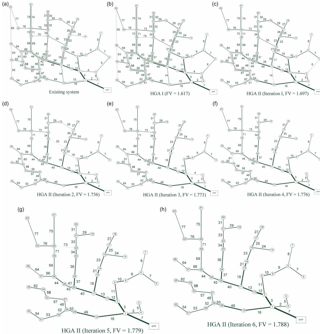
Figure 5 | Alterations to the network. Note: Diameter solution is 150 mm (pipe to be discarded for the next process).
