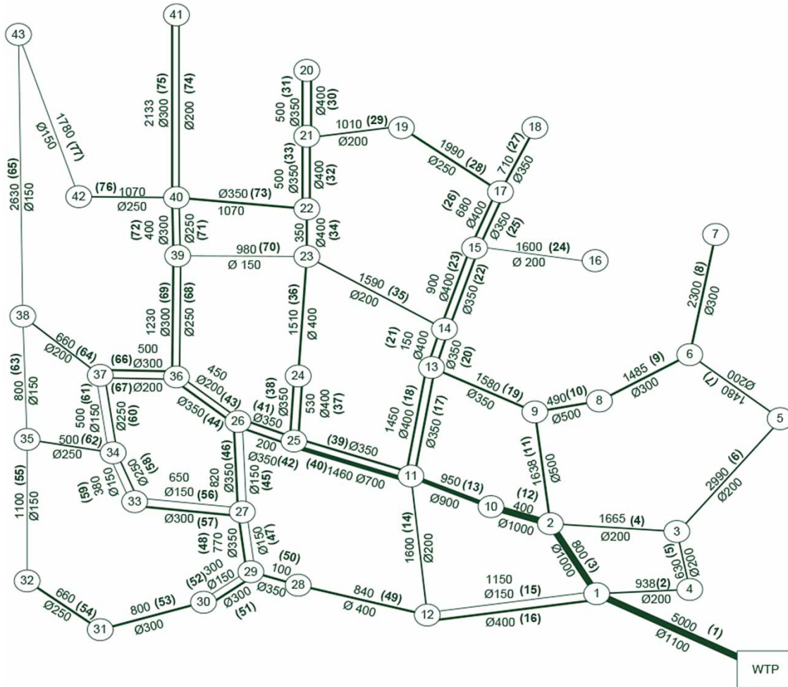
Figure 1 | Somba Opu Distribution system (network study).
