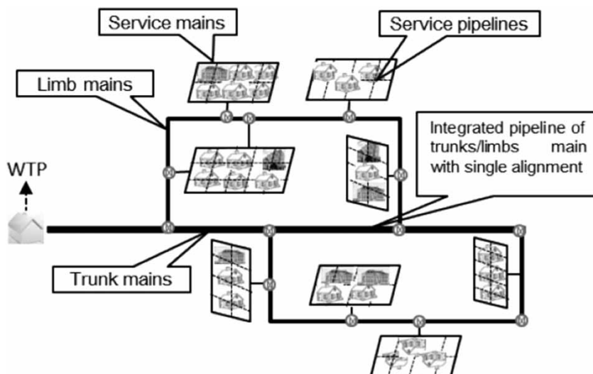
Figure 3 | Conceptual pipeline of a TMR system.
