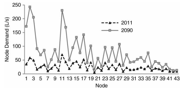
Figure 2 | Node water demand in 2011 and 2090. The total increase is expected to be three-fold.
