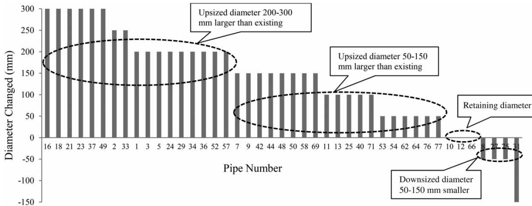
Figure 7 | Diameter changes to existing diameter derived by HGA II.
