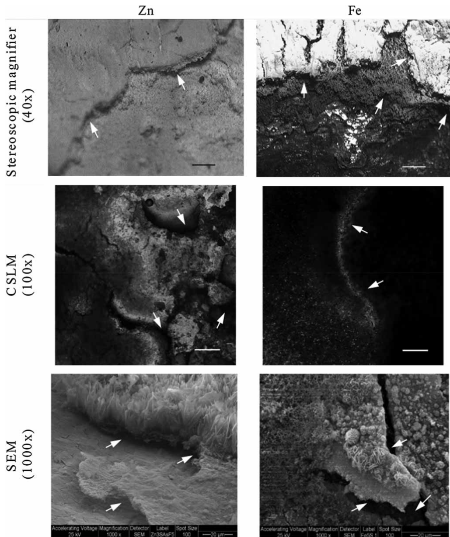
Figure 3 | Structural aspect of complex deposits on the most susceptible to colonization materials, Zn and Fe, with different image analysis equipment. Stereoscopic magnifier bar: 500 \mu\text{m} ; CSLM bar: 200 \mu\text{m} ; SEM bar: 20 \mu\text{m} . White arrows indicate different distinguishable layers.
