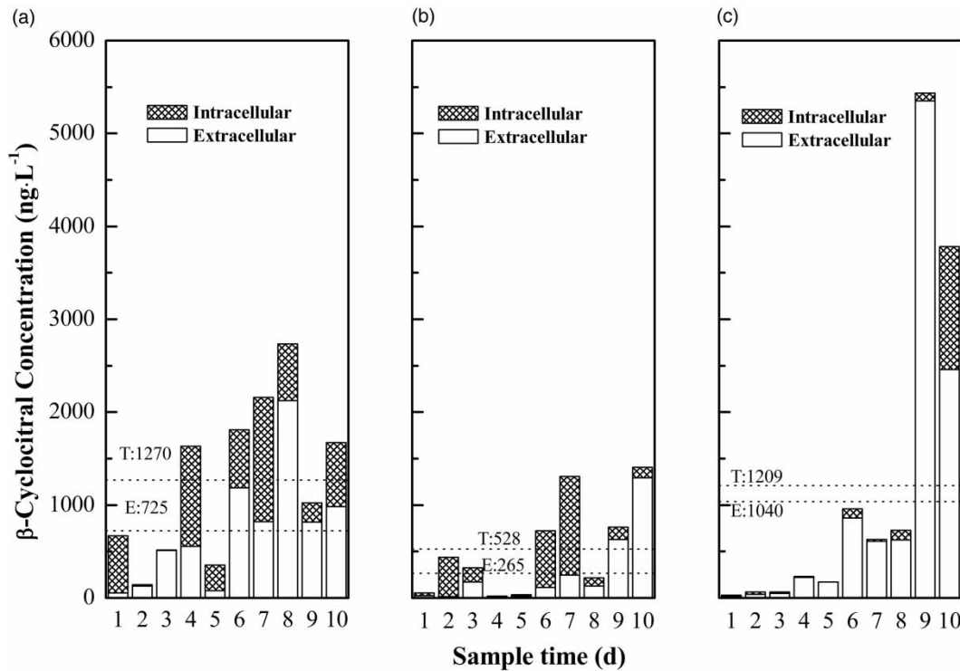
Figure 6 | Distribution of \beta -cyclocitral under different initial pH values of M. aeruginosa suspensions (initial concentration: 10^7 cells/L). (a) pH unadjusted, 12L/12D; (b) pH = 4.2, 12L/12D; (c) pH unadjusted, 24D, L, light; D, dark.
