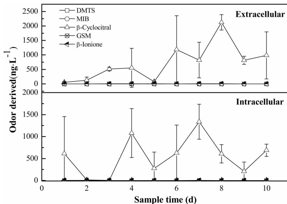
Figure 2 | Extracellular and intracellular odor contaminants with M. aeruginosa cells at a density of 10^7 cells/L.
