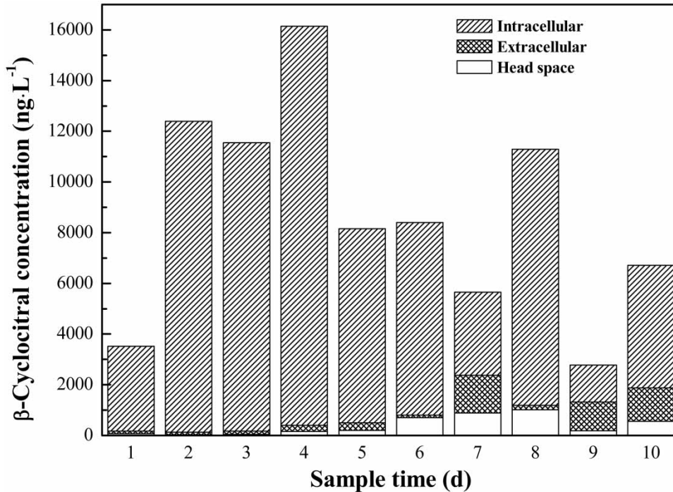
Figure 3 | \beta -Cyclocitral distribution over time for M. aeruginosa ( 10^8 cell per liter).
