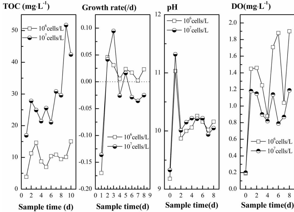
Figure 5 | Variation of pH, total organic carbon (TOC), DO and M. aeruginosa growth rate as a function of time.
