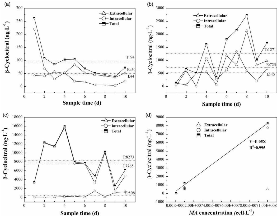
Figure 4 | \beta -Cyclocitral distribution at different cell concentrations (a) 10^6 cells/L; (b) 10^7 cells/L; (c) 10^8 cells/L.
