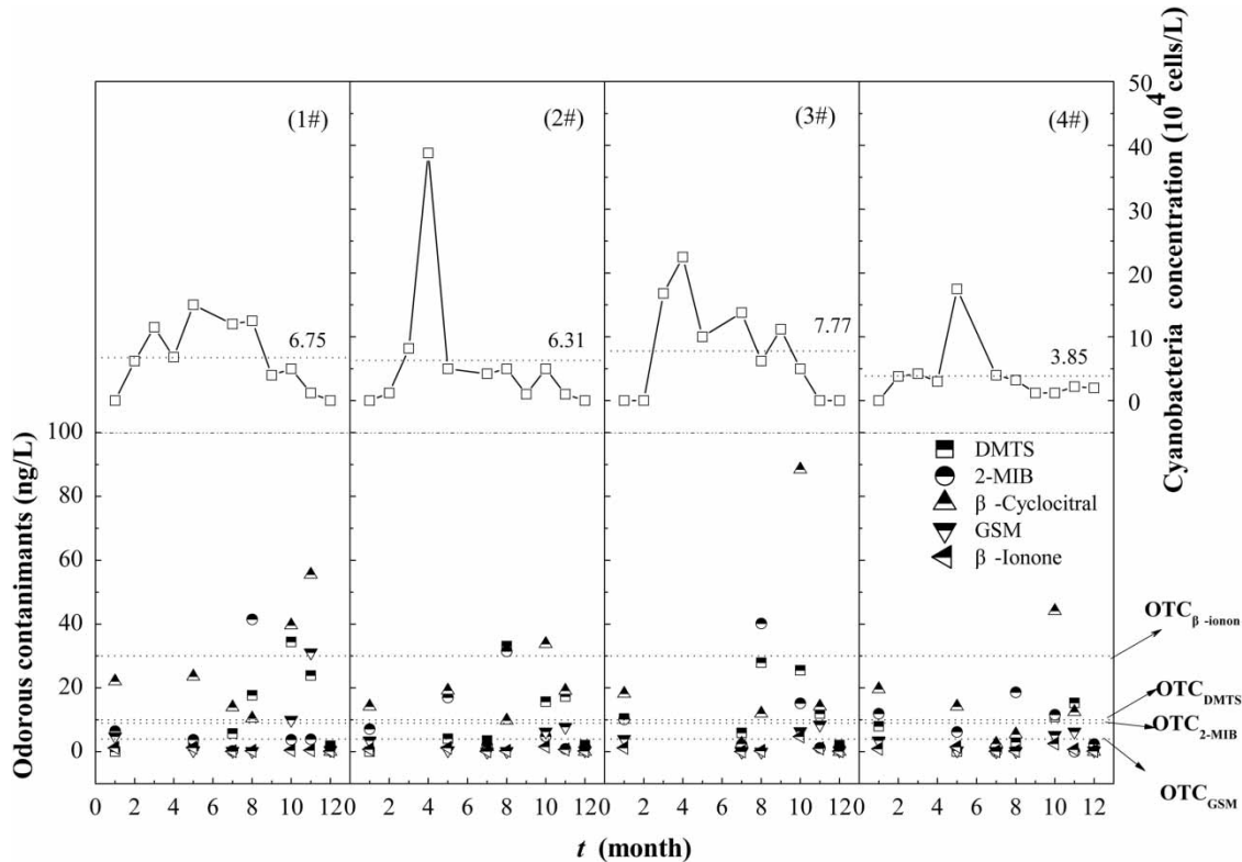
Figure 1 | Variation of cyanobacteria and odorous metabolites and DMTS at intakes to waterworks that provide drinking water for Hangzhou City. #1 and #2: Qiantang River; #3: Tiesha River; #4: Dongtiaoxi River. Dotted lines for cyanobacteria indicate the average concentration for the year. OTC of \beta -cyclocitral is 0.5–19 \mu\text{g/L} and exceeds the range shown.
