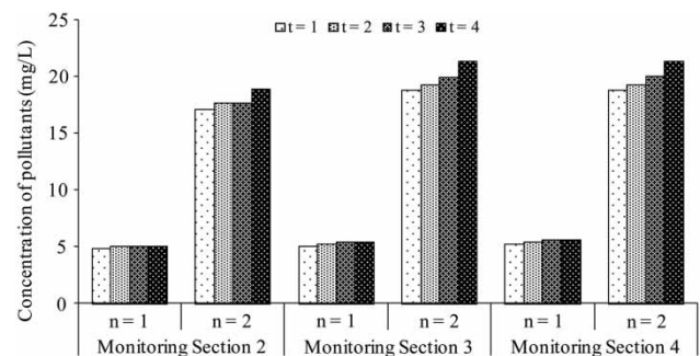
Figure 4 | BOD and COD concentrations in different monitoring sections under scenario 1.
