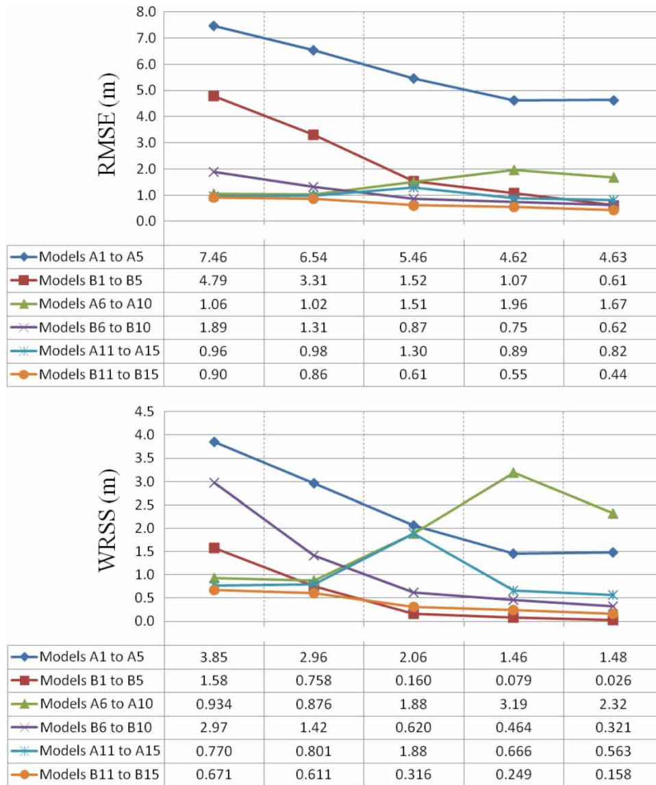
Figure 4 | RMSE and the WRSS errors for 30 models at the end of steady-state and transient modes of automatic calibration. Errors calculated between simulated and observed water levels of 18 observation wells.
