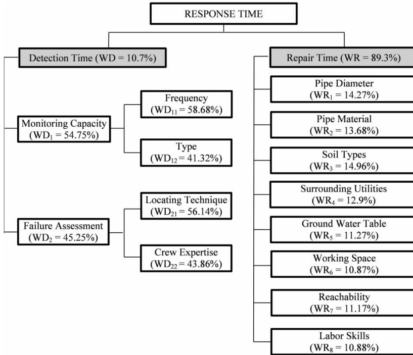
Figure 4 | Relative weightings for factors influencing response time to main breaks.
