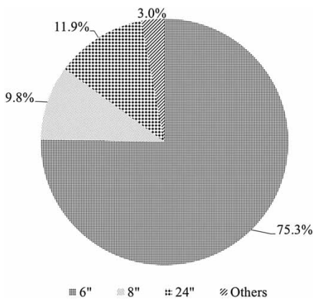
Figure 7 | Distribution of CWDN pipe diameter by length (1 inch = 25.4 mm).
