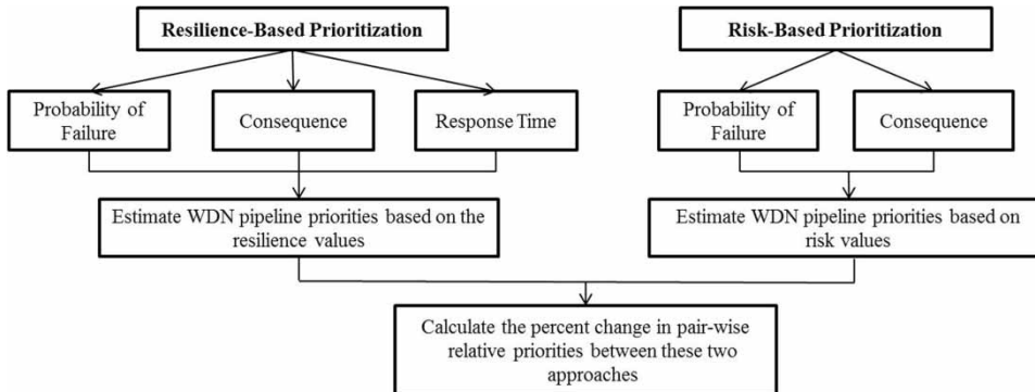
Figure 10 | Resilience- vs. risk-based prioritization comparison methodology.
