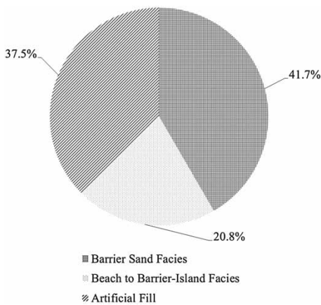
Figure 8 | Distribution of soil type in CWDN region by pipeline length.
