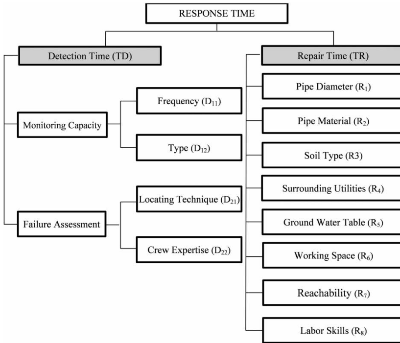
Figure 3 | Factors influencing response time to main breaks.
