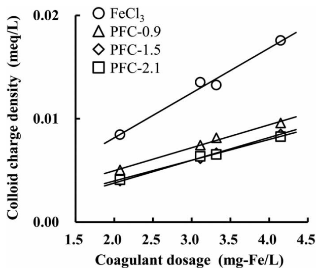
Figure 5 | Positive colloid charge densities of the PFC coagulants used in the present study as evaluated by means of a colloid titration method. The numbers after 'PFC' represent the basicity of the coagulant.
