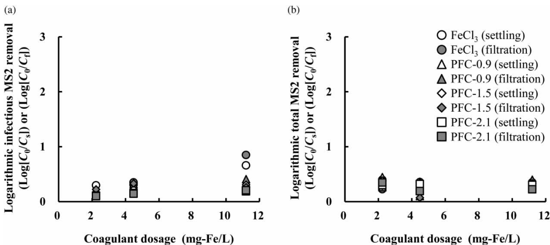
Figure 3 | Effect of the basicity and dosage of PFC on infectious MS2 removal as evaluated by using a plaque-forming unit method (a) and on total MS2 removal as evaluated by using a real-time PCR method (b) after settling and after membrane filtration at pH 8. The numbers after 'PFC' represent the basicity of the coagulant.
