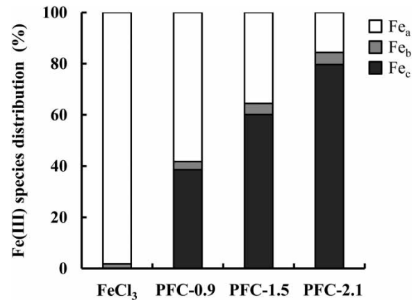
Figure 4 | Distribution of iron(III) species in the PFC coagulants used in the present study as evaluated by a ferron method. The numbers after 'PFC' represent the basicity of the coagulant. \text{Fe}_a , monomeric species; \text{Fe}_b , polymeric species; \text{Fe}_c , precipitated species.
