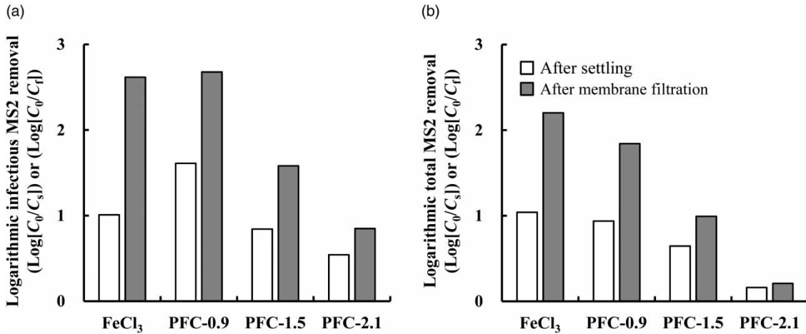
Figure 2 | Effect of the basicity of PFC on infectious MS2 removal as evaluated by using a plaque-forming unit method (a), and total MS2 removal as evaluated by using a real-time PCR method (b) after settling and after membrane filtration at pH 6. Coagulant dosage, 4.48 mg-Fe/L. The numbers after 'PFC' represent the basicity of the coagulant.
