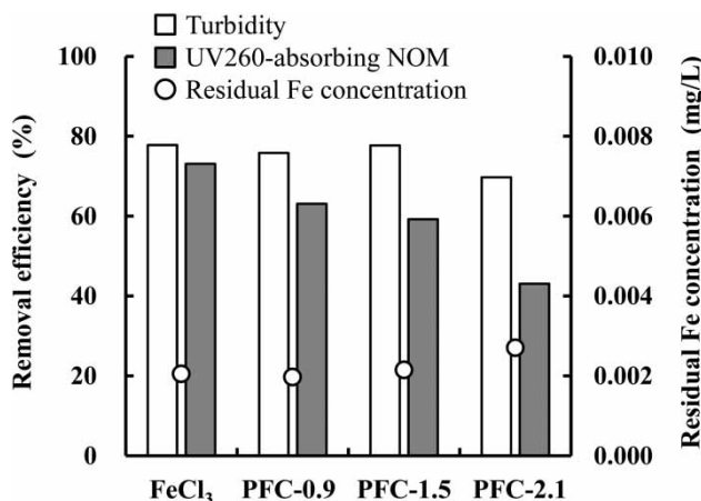
Figure 1 | Effect of the basicity of PFC on removal of turbidity and UV260-absorbing NOM, and residual Fe concentration after settling, after coagulation at pH 6. Coagulant dosage, 4.48 mg-Fe/L. The numbers after 'PFC' represent the basicity of the coagulant.
