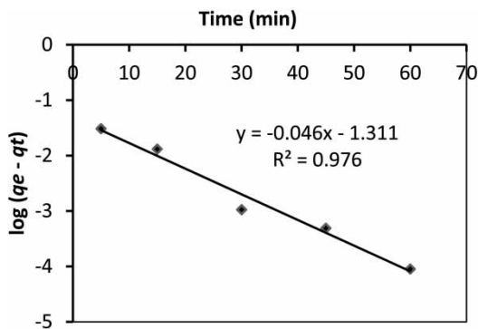
Figure 7 | First order kinetic model (adsorbent dose 10 g/L, initial concentration 0.395 mg/L, mixing speed 30 rpm).
