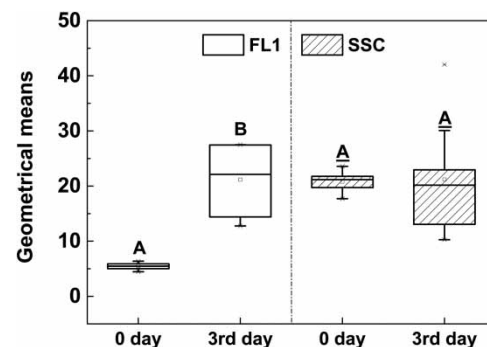
Figure 3 | The changes of green fluorescence (FL1) and side scatter (SSC) in the total bacterial community before and after 3 days' incubation. Different capital letters indicate significant difference at the 0.01 level, and letters without and with underline represent differences before and after the 3 days' incubation, respectively.
