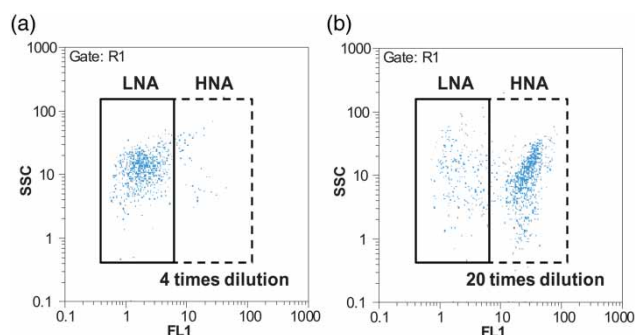
Figure 1 | Flow cytogram of LNA and HNA bacterial community (a) before and (b) after 3 days' incubation. FL1 and SSC stand for forward scatter and side scatter signal, respectively.
