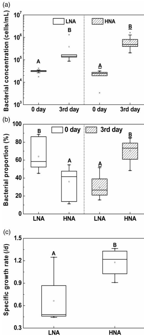
Figure 2 | The (a) concentration and (b) percentage of LNA and HNA bacteria before and after 3 days' incubation, and (c) their specific growth rate. Different capital letters indicate significant differences at the 0.01 level.
