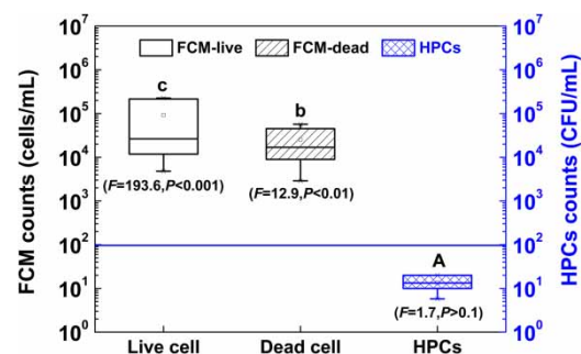
Figure 5 | Comparison of microbial biomass index between FCM and HPCs. Blue line represents the Chinese drinking water standard of total bacterial colonies. Different capital and lowercase letters indicate significant differences at the 0.01 and 0.05 levels, respectively. Please refer to the online version of this paper to see this figure in colour: http://dx.doi.org/10.2166/aqua.2017.108 .
