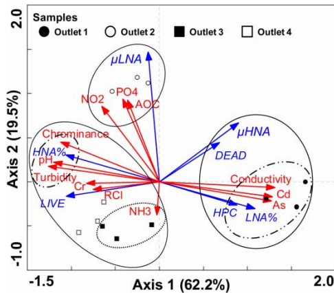
Figure 4 | Redundancy analysis plot of LNA and HNA bacterial characteristics with water physicochemical properties. Red and blue arrows represent variables of water physicochemical properties and bacterial characteristics, respectively ( \text{NH}_3 , ammonia nitrogen; \text{NO}_2 , nitrite; \text{PO}_4 , phosphate; \text{R}_{\text{Cl}} , residual chlorine; \mu\text{LNA} and \mu\text{HNA} , the specific growth rate of LNA and HNA, respectively; LIVE and DEAD, live and dead bacterial concentration; HPC, heterotrophic plate counts; LNA% and HNA%, the contribution of LNA and HNA in total FCM-bacteria, respectively). Please refer to the online version of this paper to see this figure in colour: http://dx.doi.org/10.2166/aqua.2017.108 .
