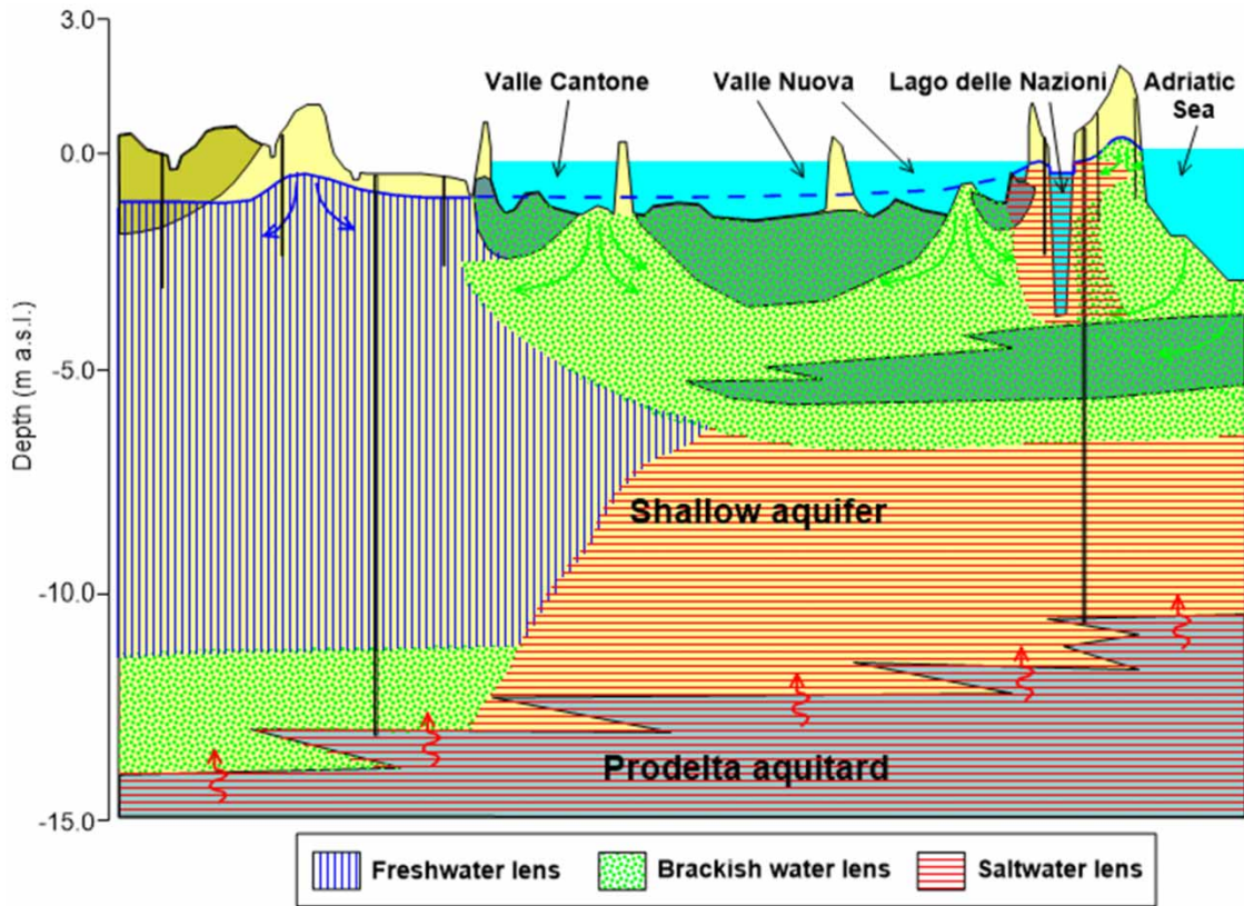
Figure 4 | The conceptual model of groundwater fluxes and salinities and their interplay with the surface water system along the AA' profile shown in Figure 1. The solid/dashed line depicts the water table and the arrows indicate the flow directions: vertical lines pattern is fresh, dotted pattern is brackish and horizontal lines pattern is saline water. The monitoring wells are represented with black lines and salinities are reported in Table 3.
