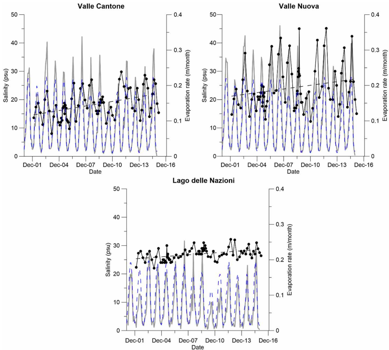
Figure 3 | Temporal trends of monthly evaporation rates calculated using Equation (1) (grey lines) and PM (dashed lines), observed lagoons' salinities (black lines and dots) and their linear trends (dashed black lines).
