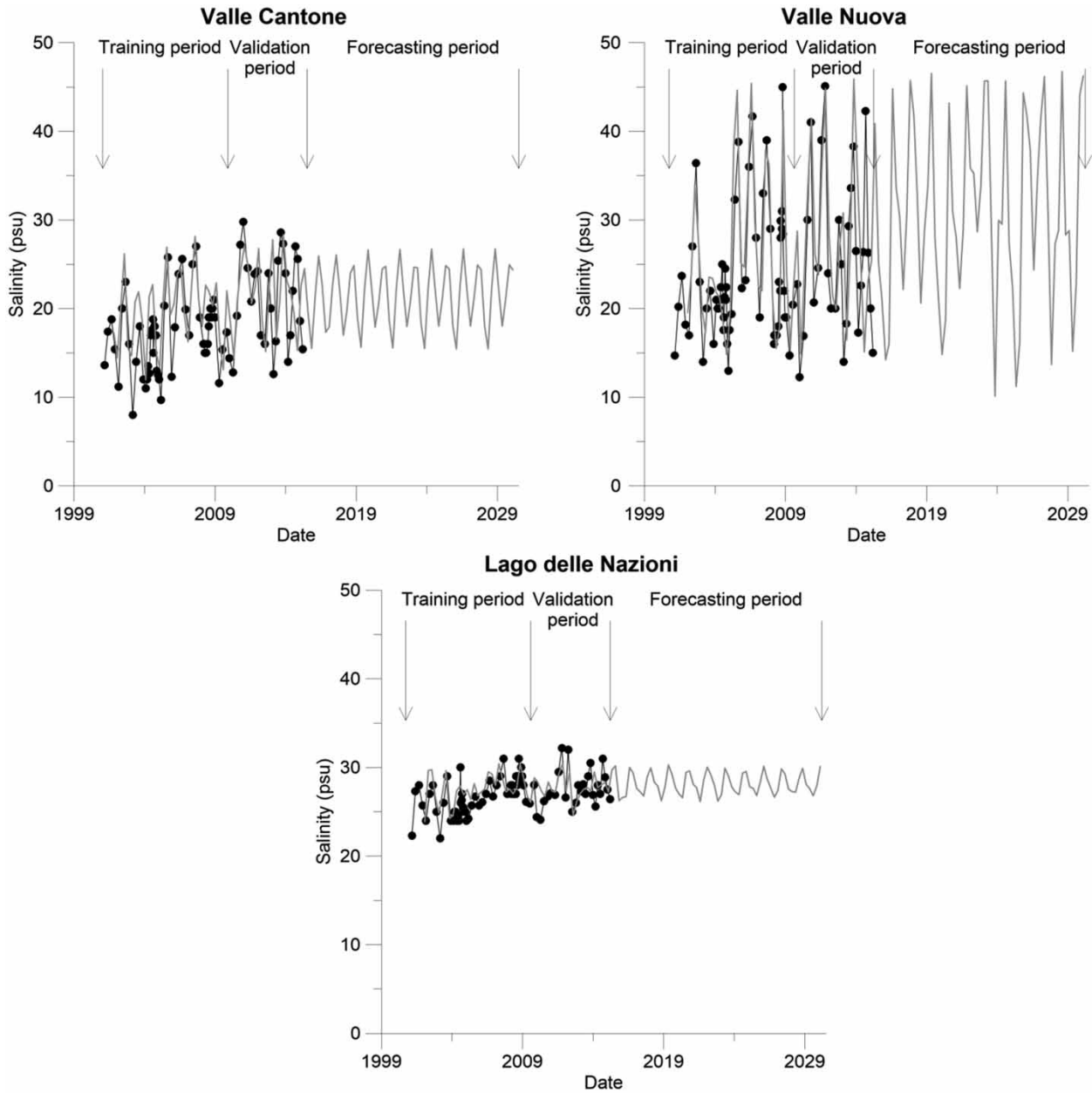
Figure 5 | Temporal trends of monthly salinities calculated by the ANN (grey lines), observed lagoons' salinities (black lines and dots); the training, validation and forecasting periods are also shown.
