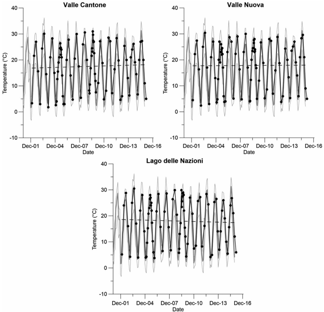
Figure 2 | Temporal trends of mean maximum and minimum atmospheric temperature (grey lines), observed lagoons' temperatures (black lines and dots) and their linear trends (dashed black lines).
