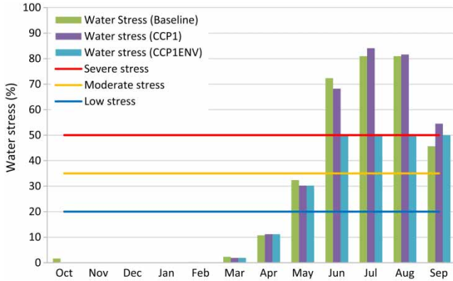
Figure 3 | Mean monthly water stress in the Ali Efenti catchment for baseline, CCP1 (future without environmental restrictions) and CCP1ENV (future with environmental restrictions) scenarios.
