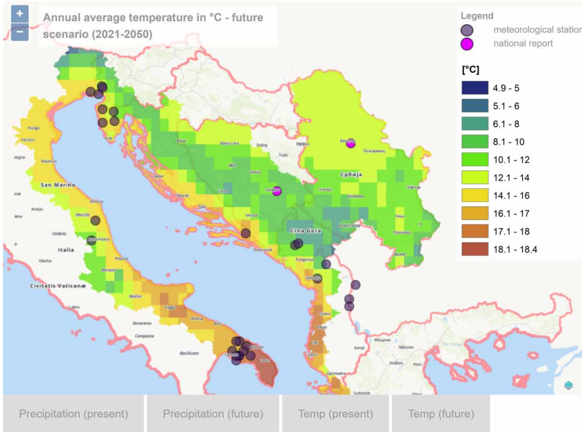
Figure 3 | DRINKADRIA web based platform – Annual average temperature in °C – future scenario (2021–2050).
