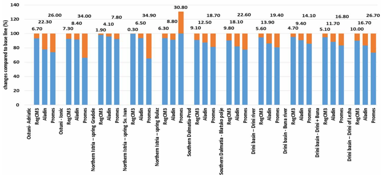
Figure 1 | Changes in average flow and recharge for future period 2021–2050 compared with 1961–1990 baseline period.
