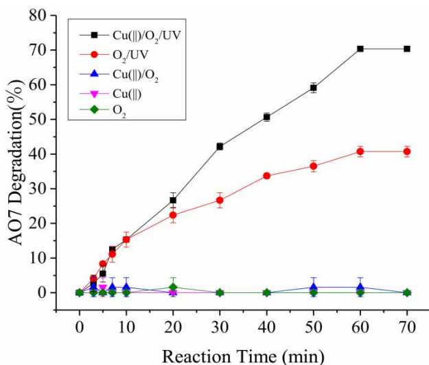
Figure 1 | Time-dependent degradation of AO7 by O 2 , Cu(II), Cu(II)/O 2 , UV/O 2 and Cu(II)/O 2 /UV processes. Experimental conditions: [Cu(II)] 0 = 10 μM, [AO7] 0 = 1.5 μM, power of UV light = 15 W, O 2 flow rate = 0.5 L·min -1 , pH = 3.5 ± 0.1, 20 °C, reaction time = 70 min.
