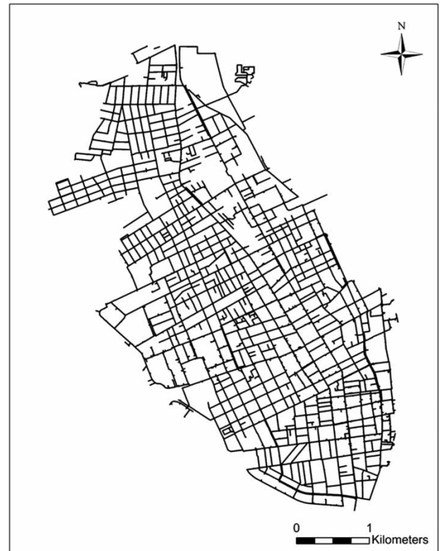
Figure 1 | Layout of the WSS in the Charleston peninsula region.
