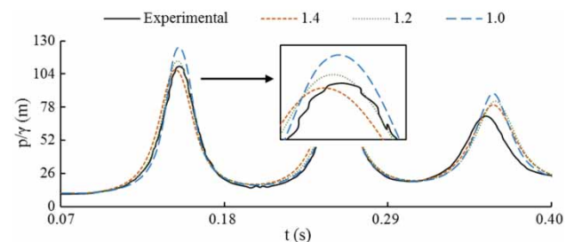
Figure 3 | Air pocket pressure versus time under different polytropic exponents.
