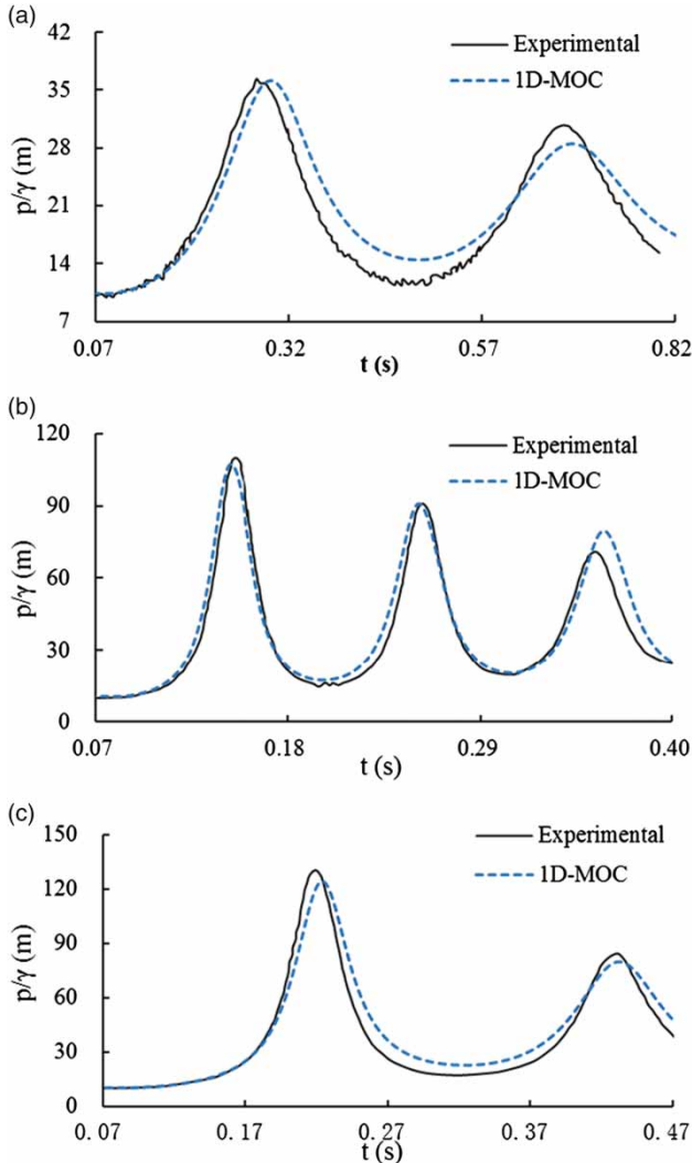
Figure 2 | Air pocket pressure comparison under three conditions: (a) condition a ( h_0 = 1 , L_{air0}/D = 9.3 ); (b) condition b ( h_0 = 1 , L_{air0}/D = 1.9 ); (c) condition c ( h_0 = 3 , L_{air0}/D = 9.3 ).
