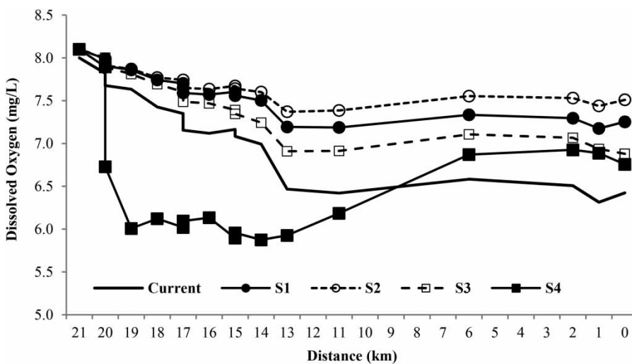
Figure 1 | DO profiles of the river under four management scenarios. S1: WLA with 45% organic matter removal; S2: WLA with 90% organic matter removal; S3: S1 with limited reuse; S4: S3 with full river water allocation.
