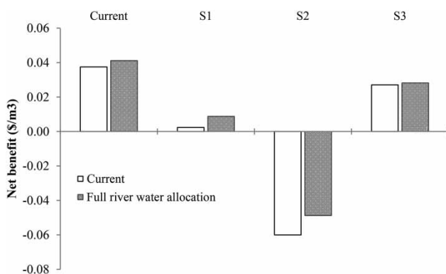
Figure 4 | Economic value of water in different scenarios in current and future horizons. S1: WLA with 45% organic matter removal; S2: WLA with 90% organic matter removal; S3: S1 with limited reuse.
